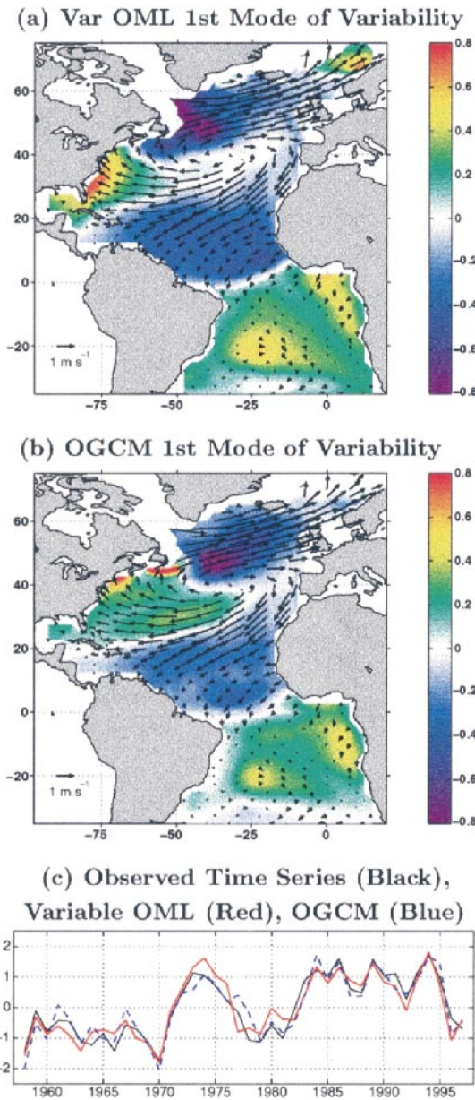
FIG. 7. Same as for Fig. 6 but for the cases where the SST anomalies were computed with a variable depth ocean mixed layer and (b) with the full dynamical ocean GCM both coupled to the AML model. The time series are shown in (c).
