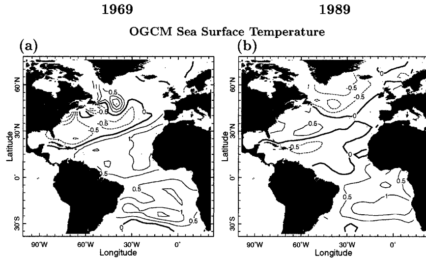
FIG. 9. The SST anomalies for Jan–Mar seasonal means as simulated by the ocean GCM for (a) 1969 and (b) 1989. These can be compared to the corresponding figures for the observed anomalies in Fig. 3.
