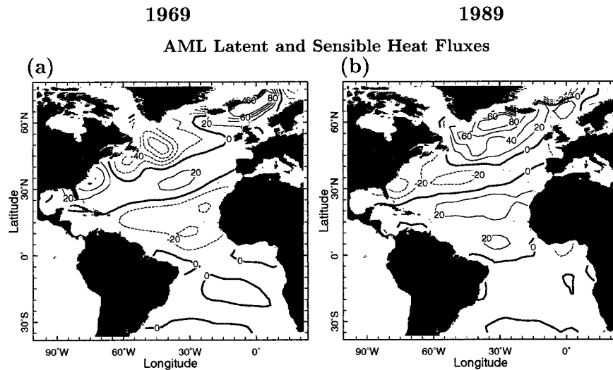
FIG. 3. The latent plus sensible heat flux anomalies in W m^{-2} simulated by the AML model when forced by NCEP–NCAR reanalyzed SSTs and winds for Jan–Mar seasonal means for (a) 1969 and (b) 1989.
