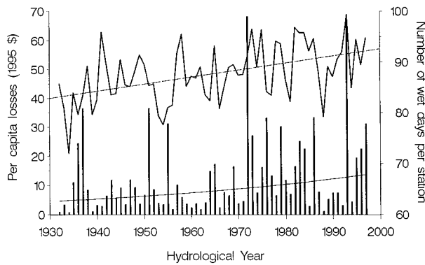
FIG. 5. (a) Two-day precipitation events superimposed on Fig. 3a, per capita damage. (b) Number of wet days superimposed on Fig. 3a, per capita damage.
