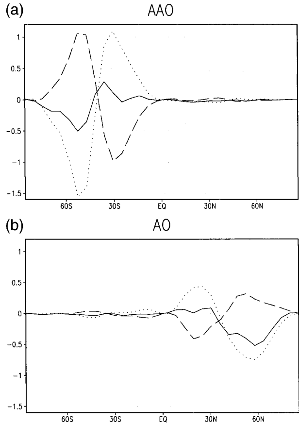
FIG. 5. Profiles of c_u(\varphi) (dashed lines), c_l(\varphi) (dotted lines), and c(\varphi) (solid lines), obtained from the regression patterns of zonal-mean meridional wind of (a) the AAO and (b) the AO. The transport of the upper branch of the meridional circulation, c_u , is obtained by performing the vertical integration \int dp in Eq. (6) from the top of the model atmosphere to 700 hPa, and the transport of the lower branch of the meridional circulation, c_l , is obtained by performing the vertical integration from 700 hPa to the surface. The unit is Hadleys.
