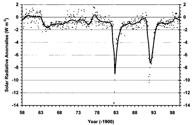
FIG. 4. Smoothed monthly mean net solar radiative forcing at Mauna Loa as derived from daily transmission and irradiance measurements described in the text. The dark solid line is the LOWESS smoother. Individual points are monthly averages.
