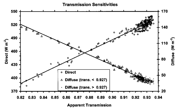
FIG. 3. Clear-sky, monthly average, direct and diffuse irradiance at Mauna Loa for zenith angle of 60^\circ from 1980 to 1998 vs apparent transmission. Plotted lines are least squares fit to the data and give the linear relationship between irradiance and apparent transmission. Note that two different lines were fit to the diffuse data above and below a transmission value of 0.927 at which apparently different scattering phase functions come into existence. Note also that some data points used in the fits are offscale to the left so that an expanded scale can be used to better display the 0.927 transmission transition region but yet show many of the lower transmission points.
