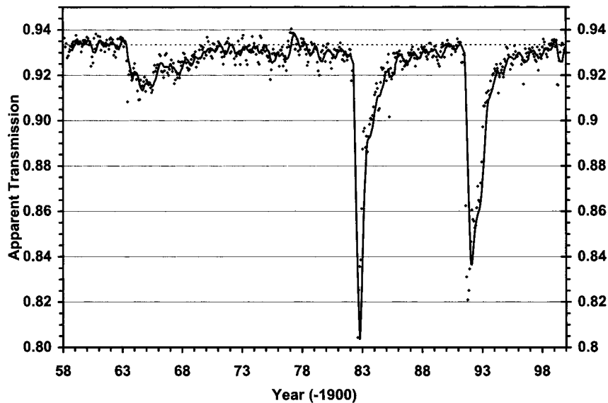
FIG. 1. Monthly average apparent solar transmission for Mauna Loa. The solid line is a 6-month LOWESS smoother, individual points are monthly averages, and the dashed line is the 1958–62 background value of 0.9335. Note that a few points are offscale (low) in 1982.
