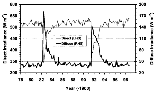
FIG. 2. Monthly average clear-sky direct and diffuse solar irradiance observed at Mauna Loa for a morning solar zenith angle of 60^\circ .
