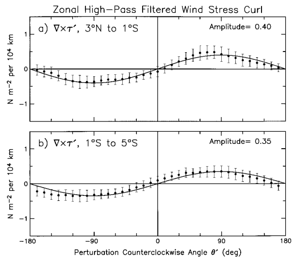
FIG. 9. The same as Fig. 8, except the angular dependencies of zonally high-pass filtered wind stress curl, \nabla \times \tau' \cdot \hat{\mathbf{k}} . The smooth curves represent least squares fits of the binned overall means to a sine.
