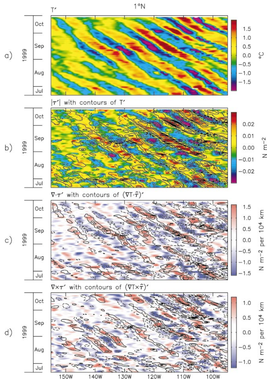
FIG. 14. Time-longitude plots along 1^\circ\text{N} on the north side of the cold tongue showing zonally high-pass filtered SST and wind stress fields: (a) perturbation SST; (b) perturbation wind stress magnitude with contours of perturbation SST overlaid; (c) perturbation wind stress divergence with contours of the perturbation downwind SST gradient, (\nabla T \cdot \hat{\tau})' , overlaid; and (d) perturbation wind stress curl with contours of the perturbation crosswind SST gradient, (\nabla T \times \hat{\tau})' \cdot \hat{k} , overlaid. Contour intervals are 0.5^\circ\text{C} in (b) and 0.4^\circ\text{C} (100 \text{ km})^{-1} in (c) and (d). For clarity, zero contours have been omitted from (b) to (d).
