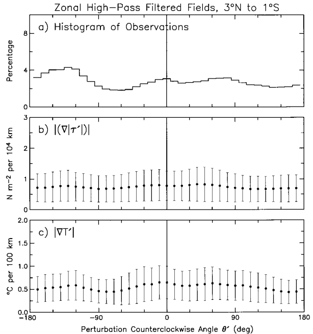
FIG. 6. The same as Fig. 5, except for the perturbation SST and wind stress fields, T' and \tau' , over the longitude range 150^{\circ} – 100^{\circ} W and the latitude range 3^{\circ} N– 1^{\circ} S on the north side of the cold tongue. The abscissa is the perturbation counterclockwise angle \theta' defined in the text.
