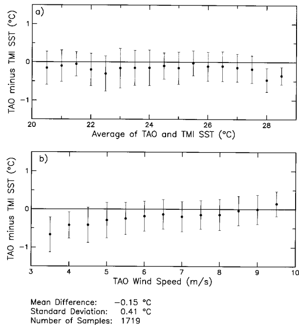
FIG. 2. Binned scatterplot comparison between 3-day averages of TMI measurements of SST and TAO measurements of temperature at a depth of 1 m at the locations shown by the solid squares in Fig. 1a. The differences between TAO and TMI measurements of temperature were binned as functions of (a) the average of the two temperature measurements; and (b) TAO measurements of wind speed. Solid circles and vertical bars represent the mean and \pm 1 standard deviation of the scatter of points within each bin.
