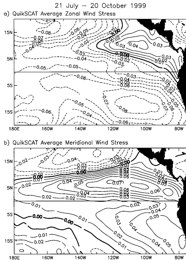
FIG. 17. Three-month averages (21 July–20 October 1999) over 4^\circ of longitude by 2^\circ of latitude constructed from QuikSCAT observations: (a) the zonal component of wind stress; and (b) the meridional component of wind stress. Contour interval is 0.01 \text{ N m}^{-2} and negative contours are shown as dashed lines in both panels.
