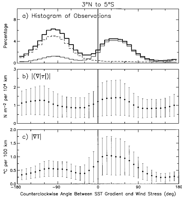
FIG. 5. Binned scatterplots of the angular dependencies of (a) the number of observations for the longitude range 150^{\circ} – 100^{\circ} W and the latitude range 3^{\circ} N– 5^{\circ} S, 3^{\circ} N– 1^{\circ} S on the north side of the cold tongue (thin solid line) and 1^{\circ} – 5^{\circ} S on the south side of the cold tongue (dashed line); (b) the magnitude of \nabla|\tau| ; (c) the magnitude of \nabla T . The abscissa is the counterclockwise angle \theta from the SST gradient vector \nabla T to the wind stress vector \tau . The solid circles and vertical bars in (b) and (c) represent the mean and \pm 1 standard deviation of the scatter of points within each bin over the latitude range 3^{\circ} N– 5^{\circ} S and the longitude range 150^{\circ} – 100^{\circ} W.
