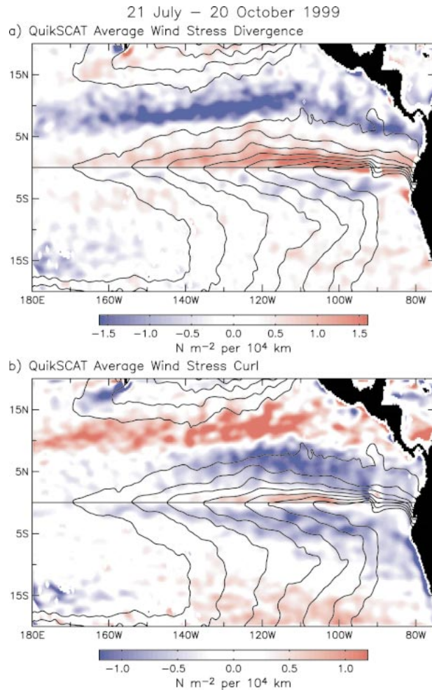
FIG. 16. Three-month averages (21 July–20 October 1999) over 4^\circ of longitude by 2^\circ of latitude constructed from QuikSCAT measurements of wind stress: (a) wind stress divergence; and (b) wind stress curl. Contours correspond to isotherms from Fig. 1a at intervals of 1^\circ\text{C} between 21^\circ and 27^\circ\text{C} .
