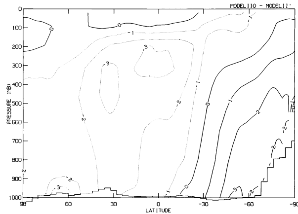
FIG. 4. Pressure–latitude cross section of temperature differences ( ^{\circ}C ) between MODELIIO and MODELII'.
