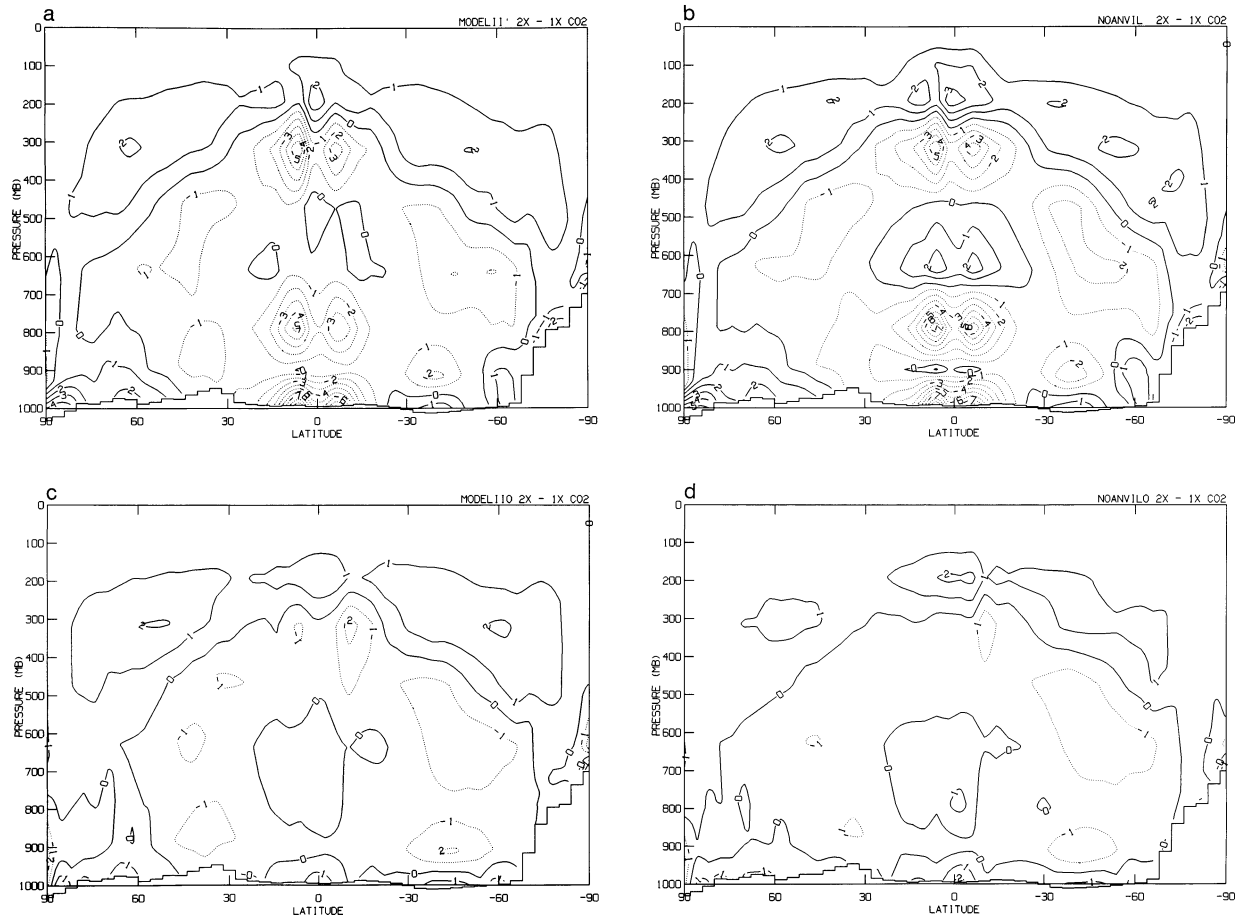
FIG. 7. Pressure–latitude cross sections of changes in total cloud cover (%): (a) MODELII', (b) NOANVIL, (c) MODELII0, and (d) NOANVILO.
