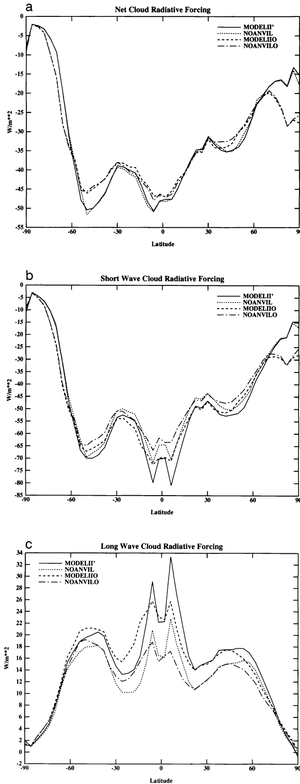
FIG. 3. As in Fig. 2, but for CRF ( W m^{-2} ): (a) net CRF, (b) shortwave CRF, and (c) longwave CRF.
