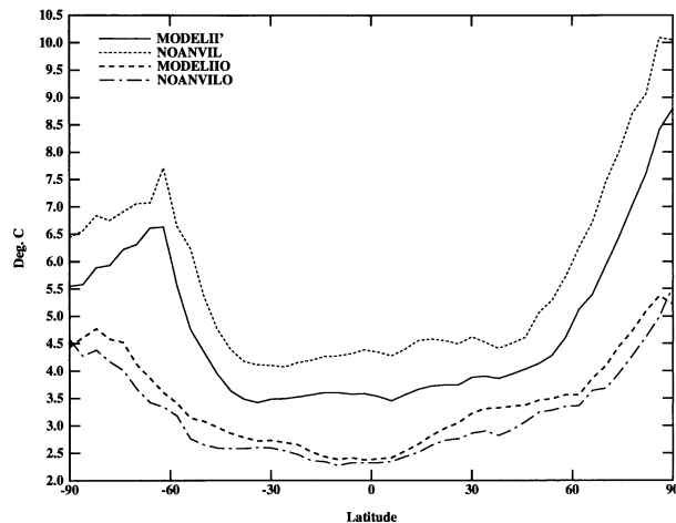
FIG. 6. Zonal mean and annual mean changes in surface air temperature ( ^{\circ}C ).
