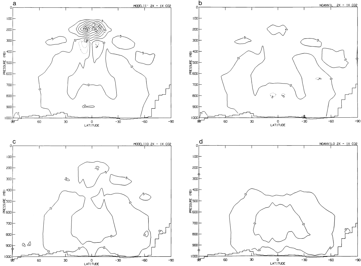
FIG. 8. As in Fig. 7, but for cloud water content ( 10^{-6} \text{ g g}^{-1} ): (a) MODELII', (b) NOANVIL, (c) MODELII0, and (d) NOANVILO.
