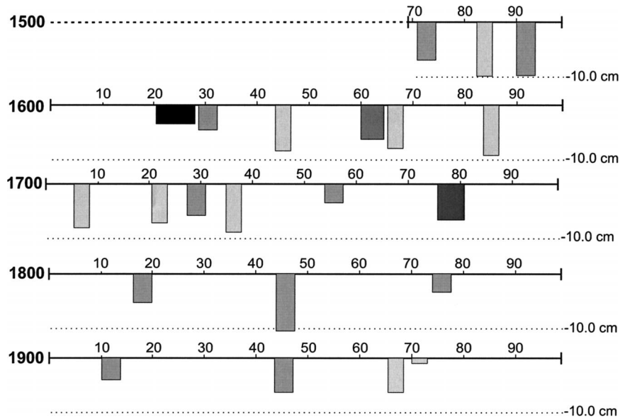
FIG. 6. Persistent low SWE events (3 yr or more with values consecutively below average) and their distribution by century (a century per row). The width and shade of the bar indicate number of years below average (3–7 yr, narrow to wide, light to dark shade), and the bar height indicates the annual average departure for the event. Light dotted lines indicate a negative departure of -10.0 cm (the full reconstruction average is 40.2 cm).
