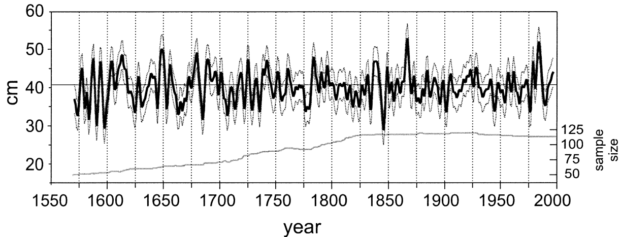
FIG. 3. Full reconstruction of Gunnison SWE, smoothed with a 5-weight binomial filter (heavy line), and error bars (thin lines), 1571–1997 (original unsmoothed years from 1569 to 1999, not shown). The thin line at the bottom of the graph indicates the change in total number of samples in the four chronologies used in the reconstruction over time (right-hand y axis).
