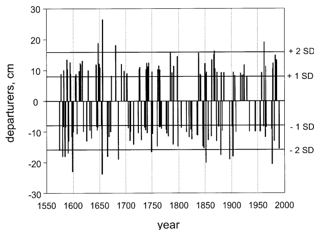
FIG. 5. Distribution of extreme years (those with values greater than \pm one std dev from average) over time. Horizontal lines above and below the zero line are one and two std dev from average.
