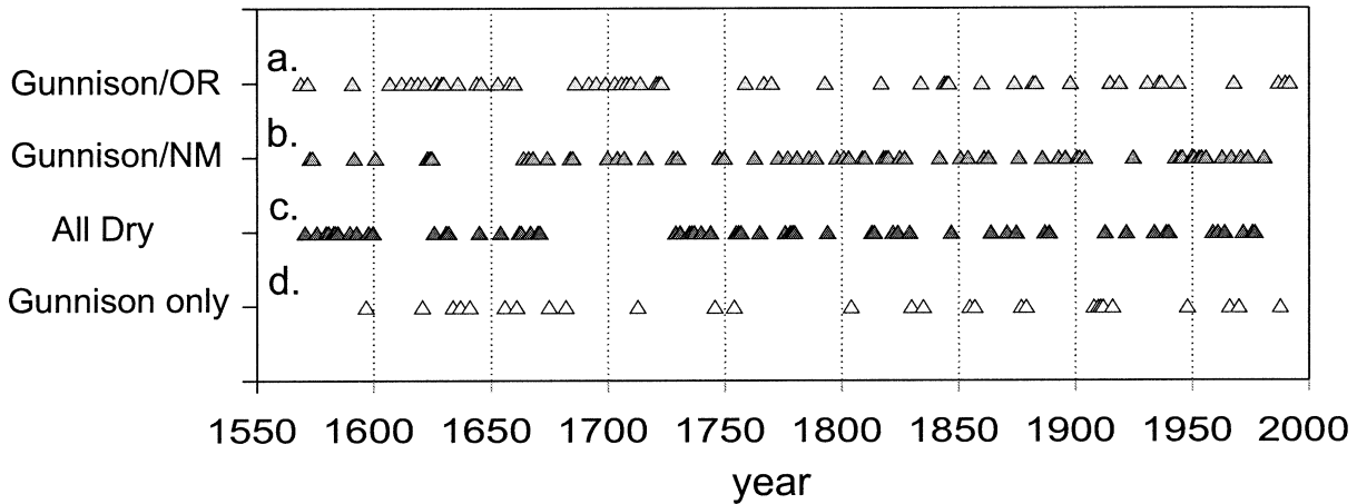
FIG. 7. Time series of years when below-average Gunnison SWE coincides with years of below average growth in (a) Oregon, (b) New Mexico, (c) in both Oregon and New Mexico, or (d) in neither Oregon nor New Mexico. Note that the top two rows represent those years when it was dry in Oregon and the Gunnison region (not in New Mexico) or dry in Oregon and the Gunnison region (not in Oregon), while the third row shows years when it was dry in all three regions.
