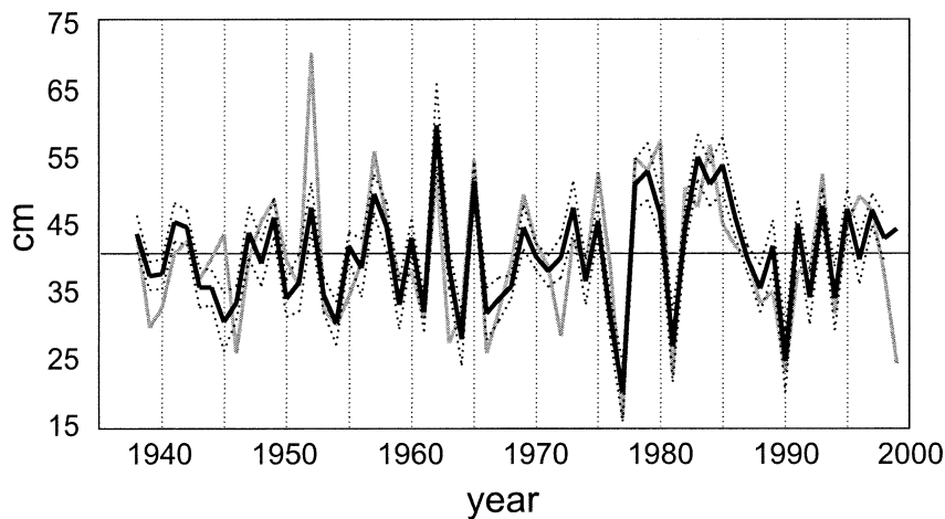
FIG. 2. Time series of observed (gray line) and reconstructed (black line) Gunnison regional SWE with 95% confidence intervals (dotted lines), 1938–99.
