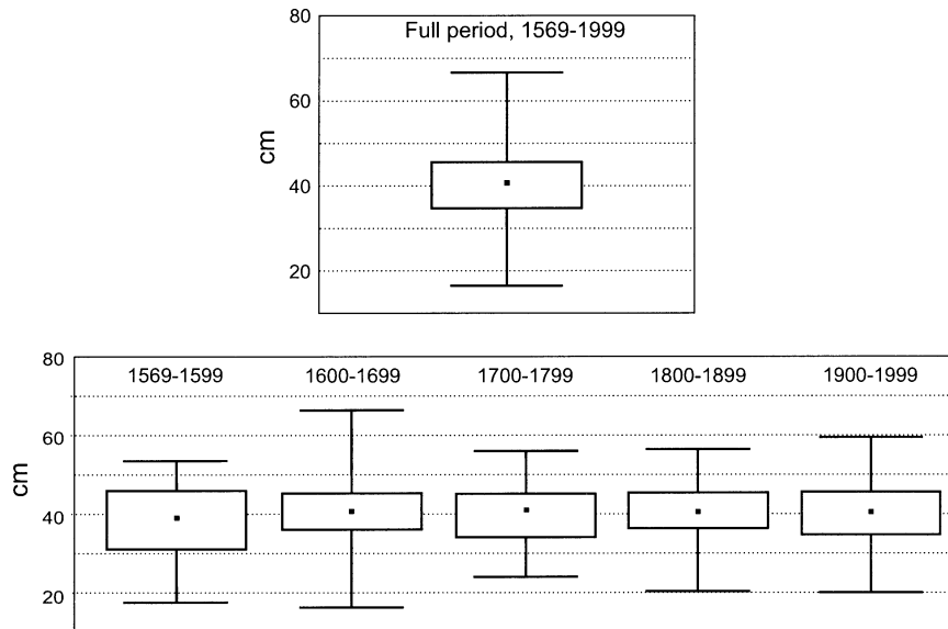
FIG. 4. Box and whisker plots for Gunnison SWE reconstruction: (top) full period and (bottom) by century (sixteenth century is 1569–99 only). The box delineates the 25th and 75th percentiles, with median (dot in box). Whiskers are max and min values.
