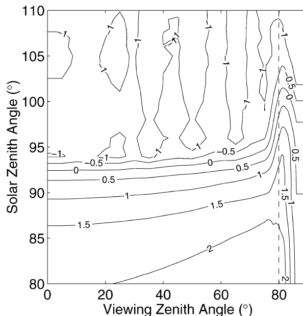
FIG. 3. Contour plot of logarithm (base 10) of the azimuthally averaged radiance derived from radiance measurements by the CERES instrument on the TRMM satellite. The viewing zenith angle is computed at 100 km above the surface. The dashed line indicates the viewing zenith angle of the tangential path to the surface of the earth.
