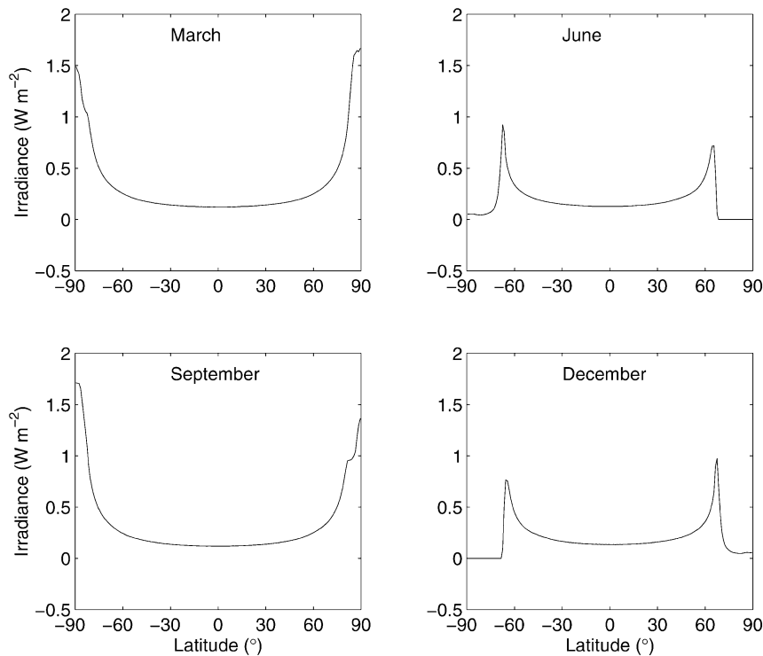
FIG. 4. Daily average twilight irradiance as a function of latitude. The relation between the irradiance and solar zenith angle shown in Fig. 2 is used to compute the daily average twilight irradiance. The positive latitude indicates the Northern Hemisphere.
