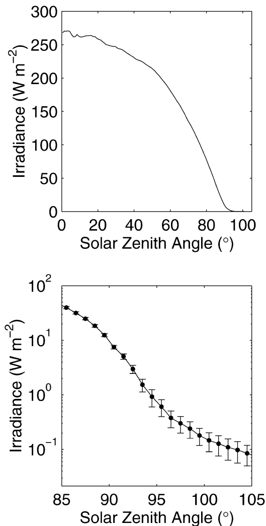
FIG. 2. Average irradiance integrated from radiances measured by the CERES instrument for the solar zenith angle from (top) 0^\circ to 105^\circ and (bottom) 85^\circ to 105^\circ . CERES data taken from Jan 1998 to Aug 1998 and Mar 2000 for all scene types were used for the computation. Two different methods for the estimate provide the error bars.
