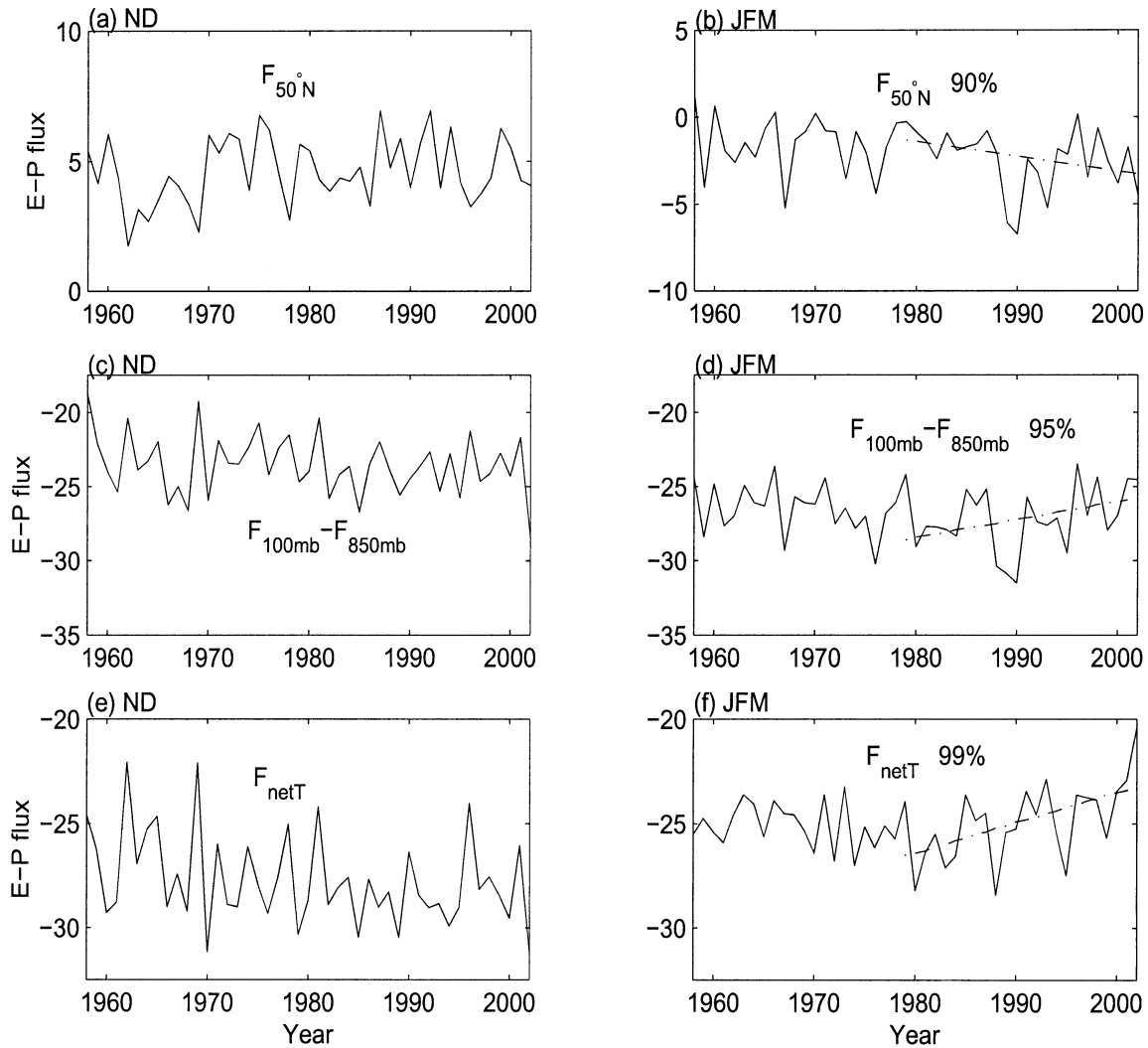
FIG. 6. The E-P flux budget in the tropospheric box. Here, F_{50^{\circ}\text{N}} is the total horizontal E-P fluxes vertically integrated from 850 to 100 mb at 50^{\circ}\text{N} ; F_{100\text{mb}} - F_{850\text{mb}} is the difference of total vertical E-P fluxes, meridionally integrated from 50^{\circ} to 90^{\circ}\text{N} , between 100 and 850 mb; F_{\text{netT}} = F_{100\text{mb}} - F_{850\text{mb}} - F_{50^{\circ}\text{N}} . The E-P flux unit is 10^{11} \text{ kg m s}^{-2} .
