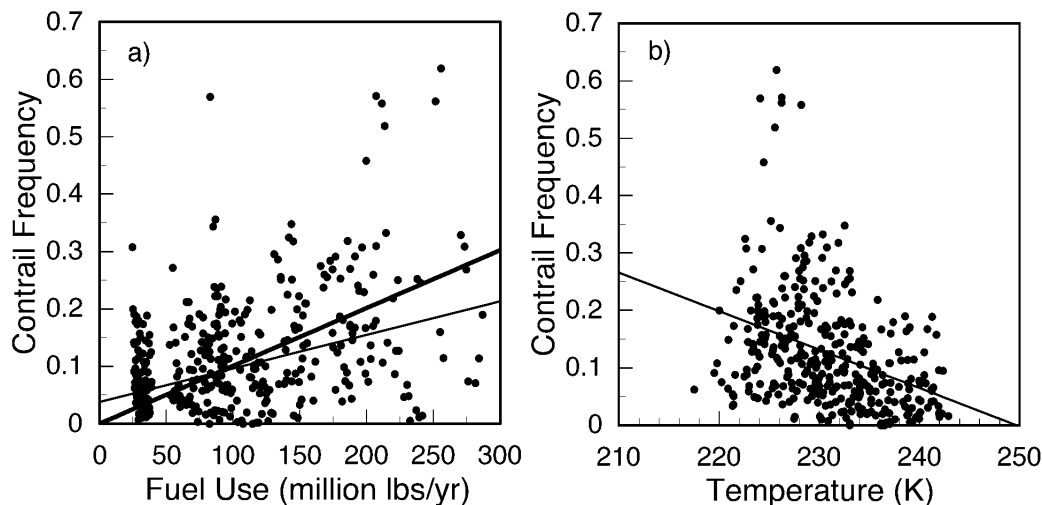
FIG. 13. Correlation of monthly mean contrail frequency and (a) estimated fuel use above 7 km and (b) 300-hPa temperatures. Thin lines indicate linear regression fit. Heavy line indicates regression fit without an intercept.
