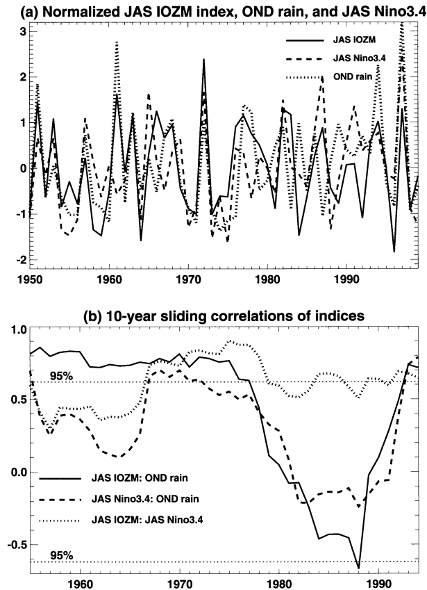
FIG. 4. (a) Time series of the normalized JAS IOZM index (solid line), the OND East African rainfall (dotted line), and the JAS Niño-3.4 index (dashed line). (b) Sliding correlations with a 10-yr window between the JAS IOZM and the OND rain (solid line), the JAS Niño-3.4 and the OND rain (dashed line), and the JAS IOZM and the JAS Niño-3.4 (dotted line). The horizontal dotted lines indicate the 95% significance level ( \pm 0.63 ).
