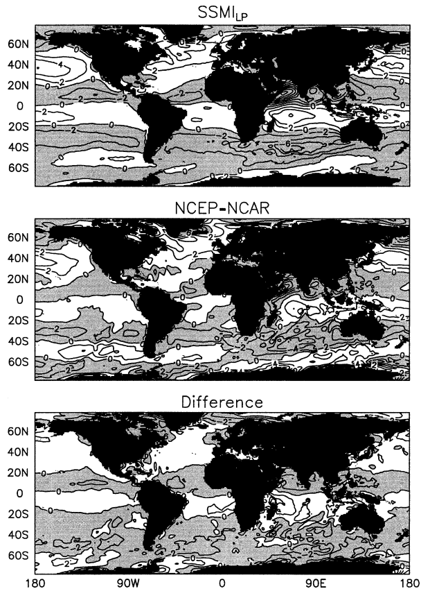
FIG. 6. Estimates of zonal wind stress \tau on the atmosphere for JJA season during 1992–99 for SSMI LP , NCEP–NCAR, and their difference (SSMI LP minus NCEP–NCAR). Annual means have been removed. Contour interval is 0.02 \text{ N m}^{-2} . Light shading denotes negative values.
