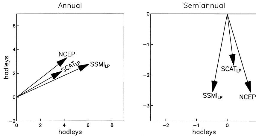
FIG. 2. As in Fig. 1 but for T_o phasors derived from NCEP–NCAR, SSMI LP , and SCAT LP series based on the period 1992–99.
