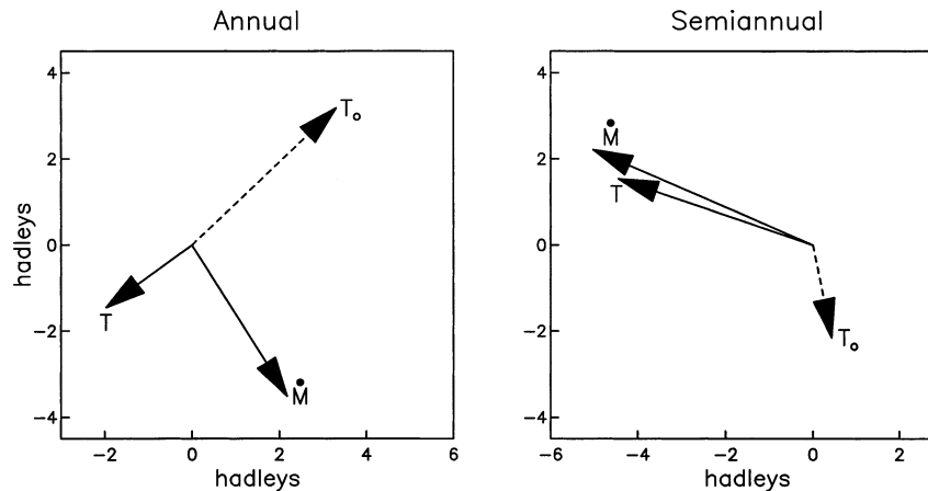
FIG. 1. Annual and semiannual amplitude and phase of \dot{M} , T , and T_o , based on NCEP–NCAR reanalysis data for 1968–98, plotted in a phasor diagram, where amplitude and phase are represented by the length and direction of a vector, respectively. Amplitudes are given in units of hadleys ( 1 \text{ hadley} = 10^{18} \text{ kg m}^2 \text{ s}^{-2} ). Phase is plotted increasing counterclockwise, with 90^\circ given by a phasor pointing straight upward. A phase of 0^\circ corresponds to an annual maximum on 1 Jan or semiannual maxima on 1 Jan and \sim 6 months later.
