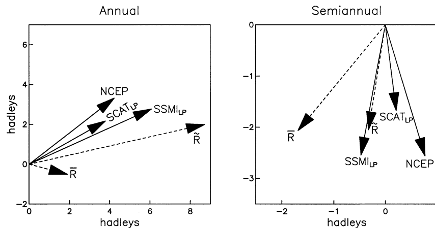
FIG. 7. Comparison of the estimates of T_o with the residual R = \bar{M} - T_L , calculated for the period 1992–99. Phasor with T_{\text{gw}} included is denoted by \tilde{R} ; phasor without T_{\text{gw}} is denoted by \bar{R} .
