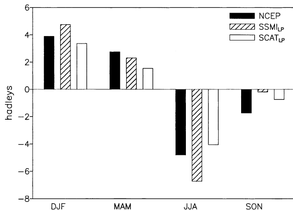
FIG. 3. Seasonal averages of NCEP–NCAR, SSMI LP , and SCAT LP estimates of T_o for the period 1992–99. The x -axis labels denote the three months of each season [e.g., Dec–Jan–Feb (DJF)]. Annual means have been removed.
