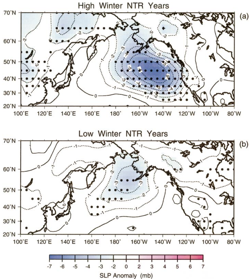
FIG. 12. Composites of winter (DJF) SLP anomalies for post-1900 extremes of (a) high and (b) low winter NTR. Winters included are the top ( n = 14 ) and bottom ( n = 15 ) 10% of winter extreme NTR in Fig. 7. Low pressure (dashed contours) and high pressure (solid contours) anomalies show the dominant extreme winter patterns. Grid locations whose composite anomaly is significantly different from the null hypothesis at \geq 95\% confidence are designated by dots.
