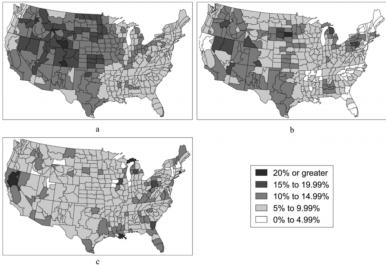
FIG. 11. The frequency at which (a) the original PDSI, (b) the CPC's PDSI, and (c) the SC-PDSI programs reported a severe or extreme drought (i.e., the percent of time the PDSI was at or below -3.0 ) at each climate division.
