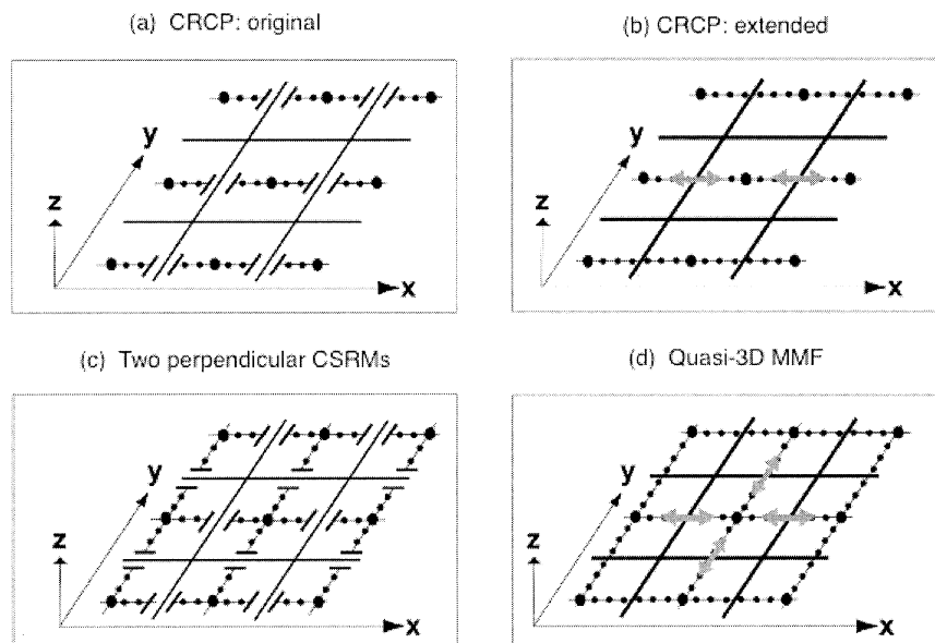
FIG. 13. (a) An illustration of the framework used in Grabowski's CRCP. (b) Same as in (a) but for a revised version in which a GCM and a 2D CRM are coupled at the large dots for scalar variables and at the arrows for velocity components. (c) Same as in (a) but for a revised version in which two perpendicular CRMs are embedded into a GCM grid box. (d) An illustration of a quasi-3D MMF.
