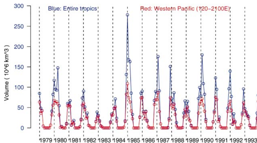
FIG. 3. Dehydration volume based on ERA-15 monthly mean temperatures. The blue curve is DV for the entire Tropics and the red curve is for the western Pacific ( 120^\circ – 210^\circ\text{E} ).
