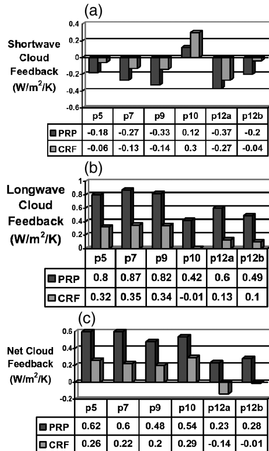
FIG. 2. Comparison of the (a) shortwave, (b) longwave, and (c) net cloud feedback parameters for the PRP and CRF methods.
