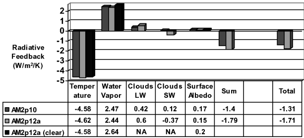
FIG. 1. Comparison of total-sky feedback strengths between AM2p10 and AM2p12a. Also shown are the clear-sky feedback strengths from AM2p12a for temperature, water vapor, and surface albedo.
