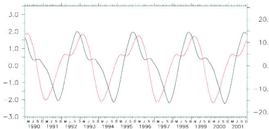
FIG. 11. Simulated Niño-3 SSTA (black) for \delta = 1.5, \gamma = 1.0 , and zonally (over whole Pacific basin) and meridionally (from 2.5^{\circ}\text{S} to 2.5^{\circ}\text{N} ) averaged thermocline depth anomaly (red).
