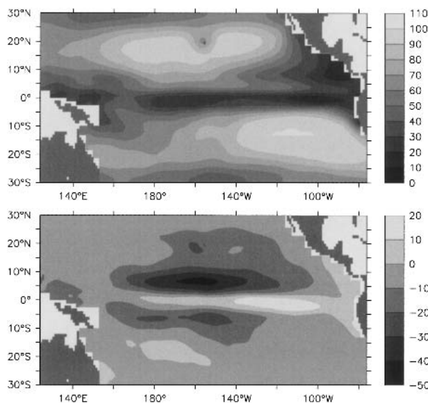
FIG. 6. (top) Mean mixed layer depth (m) for \gamma = 0 ; (bottom) MLD ( \gamma = 1.0 ) - MLD( \gamma = 0 ) (m). Here, \delta is chosen to be 1.5.
