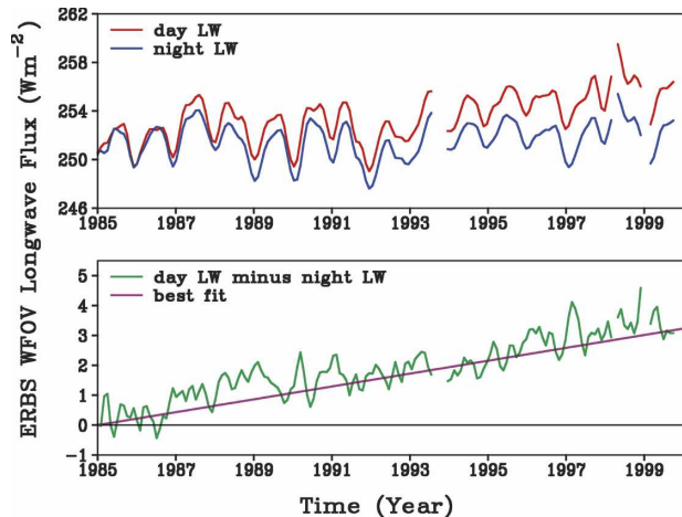
FIG. 3. Time series of ERBS Nonscanner WFOV Edition3 tropical mean ( 20^{\circ}\text{N} to 20^{\circ}\text{S} ) (top) daytime longwave flux (red curve) and nighttime longwave flux (blue curve), and (bottom) day-minus-night longwave flux differences (green curve) from 1985 to 1999.
