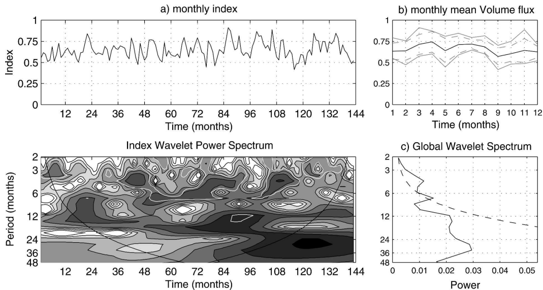
FIG. 9. (a) Monthly time series of the index for the second run and wavelet analysis of this time series; the 95% significance levels are shown by white contours and cone of influence by black line. (b) The monthly mean value of R (black line) together with the maximum (top line) and minimum (bottom line) values and one std dev above and below the mean (gray dashed lines). (c) Power of the wavelet analysis significance is shown by the dashed line. The first 60 months are considered the adjustment period of the second run.
