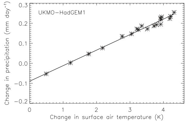
FIG. 6. Change in annual-mean global-mean precipitation rate ( \text{mm day}^{-1} ) as a function of annual-mean \Delta T for HadGEM1 forced by 2 \times \text{CO}_2 . The line is the regression and the symbols are annual means.
