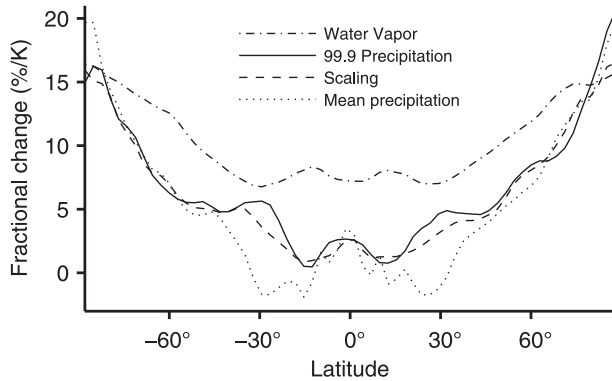
FIG. 2. Fractional changes between the reference simulation ( \alpha = 1 ) and a warmer simulation ( \alpha = 1.4 ) expressed as a percentage of the reference simulation values: column water vapor (dash-dotted), 99.9th percentile of daily precipitation (solid), precipitation extremes scaling (4) (dashed), and mean precipitation (dotted). The changes are normalized by the global-mean surface temperature difference of 6.1 K between the two simulations. The changes shown for the 99.9th percentile precipitation and the scaling have been smoothed in latitude with a 1–2–1 filter.
