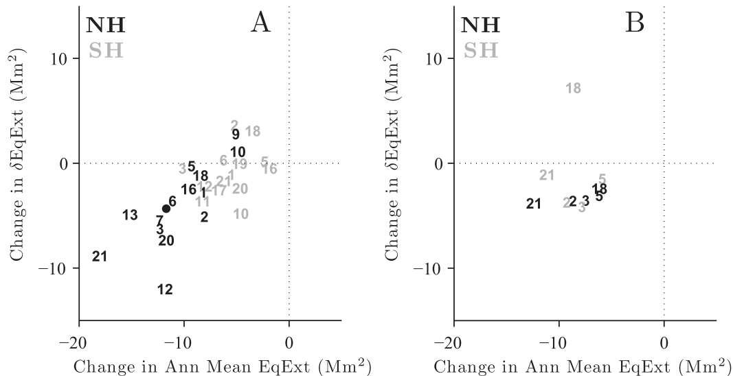
FIG. 7. Influence of edge effects and ocean dynamics on robustness among models. (a) As in Fig. 6 except that, for each hemisphere, models with ice extent less than 0.1 \text{ Mm}^2 at any time during 1900–2100 are excluded. (b) As in Fig. 6, but considering atmosphere-only equilibrium climate sensitivity simulations rather than coupled atmosphere–ocean transient simulations (see appendix B). Here, the differences between the climate under doubled \text{CO}_2 and the control simulation are plotted.
