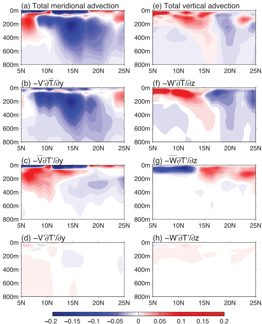
FIG. 9. Regression of advection terms ( 10^{-8}^{\circ}\text{C s}^{-1} ) onto the normalized AMO index. The regression is the ensemble mean of 12 CMIP5 models that simulate the TNA surface and subsurface temperature variation reasonably well. Shown are the (a) total meridional temperature advection, (b) advection by the anomalous meridional current, (c) advection by the mean meridional current, and (d) nonlinear term. (e)–(h) As in (a)–(d), but for the vertical temperature advection.
