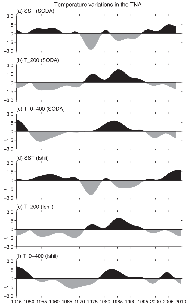
FIG. 2. Multidecadal time series of TNA (8°–20°N, coast to coast) ocean temperature anomalies at the sea surface and 200 m and vertically averaged temperature anomalies from 0 to 400 m using the (a)–(c) SODA and (d)–(f) Ishii data. All time series are normalized by their standard deviations.
