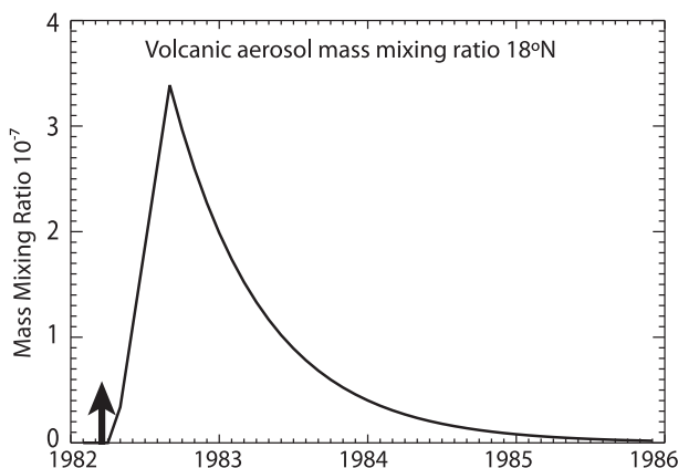
FIG. 3. The profile of aerosol mass mixing ratio in the stratosphere for the El Chichón eruption in the 1980s averaged at 18^\circ\text{N} from the CCSM4 run. The time of the eruption is given by the thick arrow and the subsequent evolution is specified in an idealized manner as to the meridional spread and time of peak and subsequent decay based on Ammann et al. (2003).
