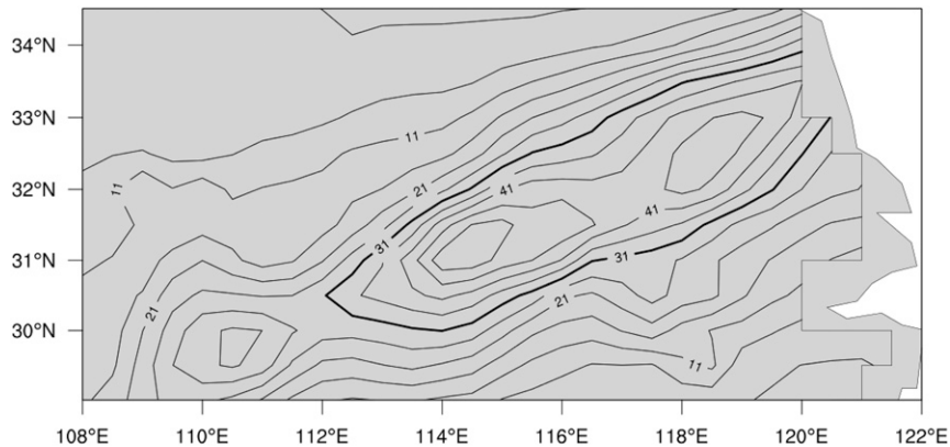
FIG. 2. The contours of the rainfall averaged over the period from 30 Jun ( M ) to 11 Jul ( N ), the period of the detected most extreme event during the rainy season. The contour corresponding to the maximal relative intensity R_3(M, N, K) ( = 391.6 \text{ mm day}^{-1} ), with its value K being 31 \text{ mm day}^{-1} , is thickened.
