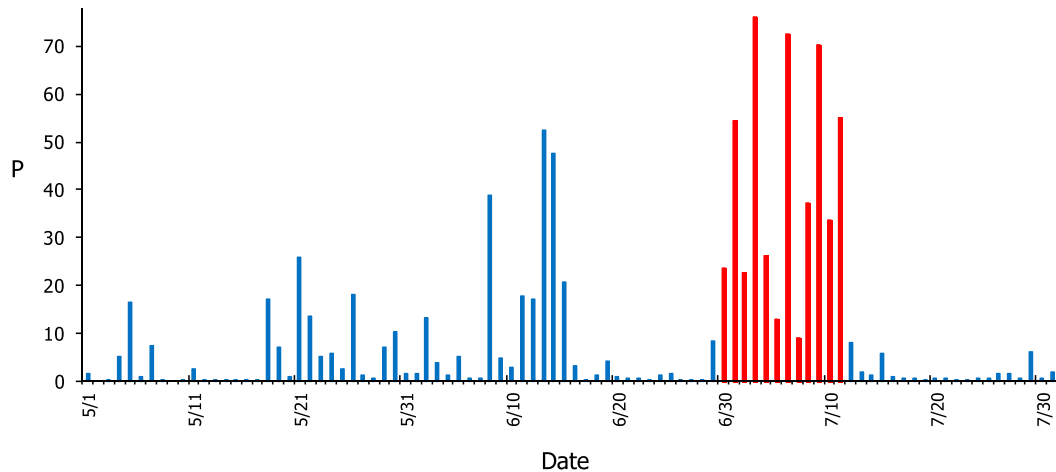
FIG. 4. The daily rainfall ( P ; \text{mm day}^{-1} ) averaged over the identified region, the one enclosed by the contour K ( =31 \text{ mm day}^{-1} ) in Fig. 2. The red bars are for the period from 30 Jun ( M ) to 11 Jul ( N ), the detected period of the most extreme event during the rainy season.
