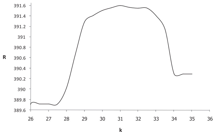
FIG. 3. The variation of the relative intensity R(M, N, k) ( \text{mm day}^{-1} ) with the value of contour k ( \text{mm day}^{-1} ). The contours of the rainfall averaged over the period M, N are displayed in Fig. 2.
