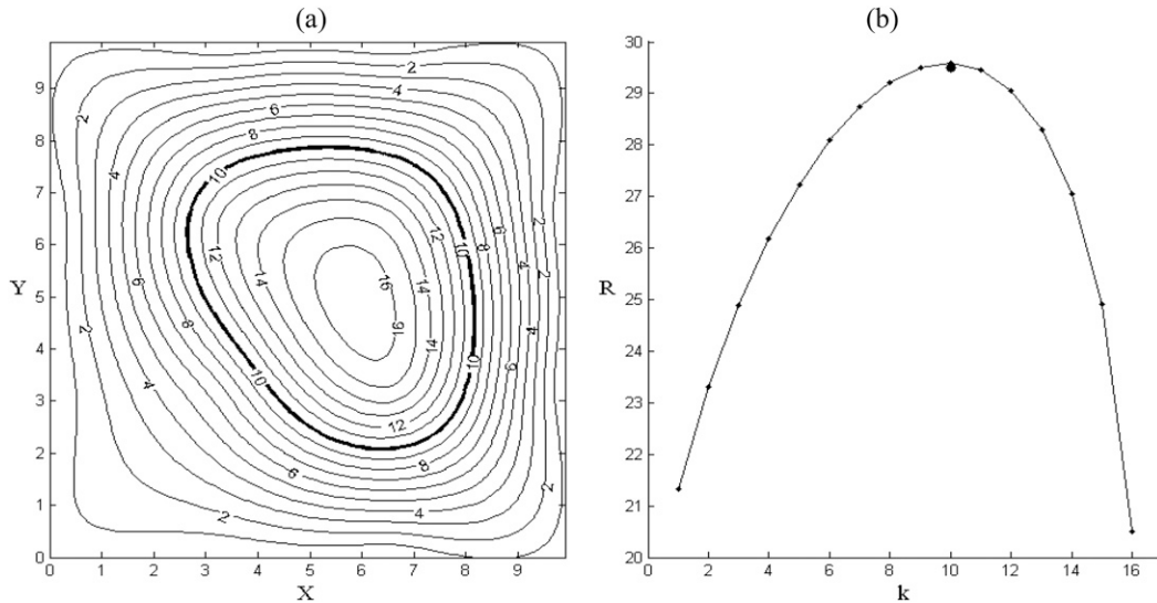
FIG. 1. A conceptual example of determining the geographic region of the extreme, from the spatial distribution of the precipitation that is averaged over a certain time period. (a) The contours indicate the distribution of the rainfall over the domain, in which X and Y both range from 0 to 10, with a resolution of 0.1 (appropriate units can be given to the rainfall and the distance). The contours are obtained through the extrapolations among a given 4 \times 4 matrix, with the four rows of the matrix being from top to bottom (0,0,0,0) , (0,15,14,0) , (0,7,12,0) , and (0,0,0,0) . The contours finally range from 0, which is along the four borders of the domain, to 16, which is the innermost contour. (b) The curve presents the value of the relative intensity R corresponding to the value of each of the contours k in (a).
