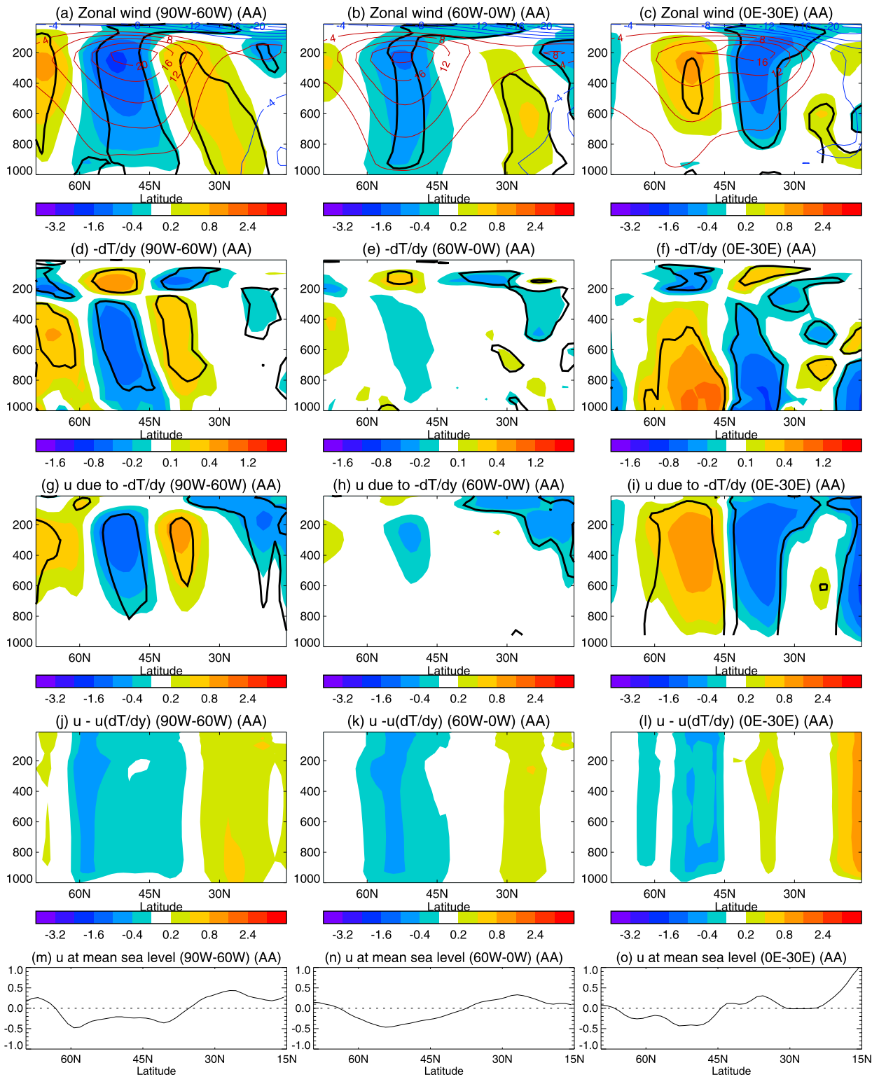
FIG. 7. Simulated (a)–(c) zonal wind changes ( \text{m s}^{-1} ), (d)–(f) meridional temperature gradient ( \text{K per } 1000 \text{ km} ), (g)–(i) zonal wind changes from the thermal wind balance related to meridional temperature gradient, (j)–(l) zonal wind change residual, and (m)–(o) geostrophic zonal wind changes at mean sea level from SLP changes for the three sectors 90^{\circ}\text{--}60^{\circ}\text{W} , 60^{\circ}\text{--}0^{\circ}\text{W} , and 0^{\circ}\text{--}30^{\circ}\text{E} in response to changes in AA (SSTAA – SST). Thin red (westerly) and blue (easterly) lines (a)–(c) are the climatology of the CON simulation. Thick lines highlight regions where differences are statistically significant at 10% level based on the two-tailed Student's t test.
