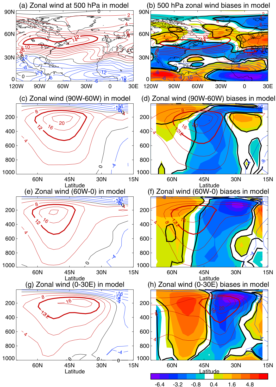
FIG. 4. (a) Model simulated climatological zonal wind ( \text{m s}^{-1} ) over the period 1964–81 at 500 hPa, and at three zonal sectors of (c) 90°–60°W, (e) 60°–0°W, and (g) 0°–30°E in JJA. (b), (d), (f), (h) Zonal wind biases (color) (CON – reanalysis) with zonal wind based on the NCEP reanalysis in contours. Thick black lines in the right column highlight regions where differences are statistically significant at 10% level based on the two tailed Student’s t test. Note that the color scales for biases are doubled in comparison with those in observed changes shown in Fig. 2.
