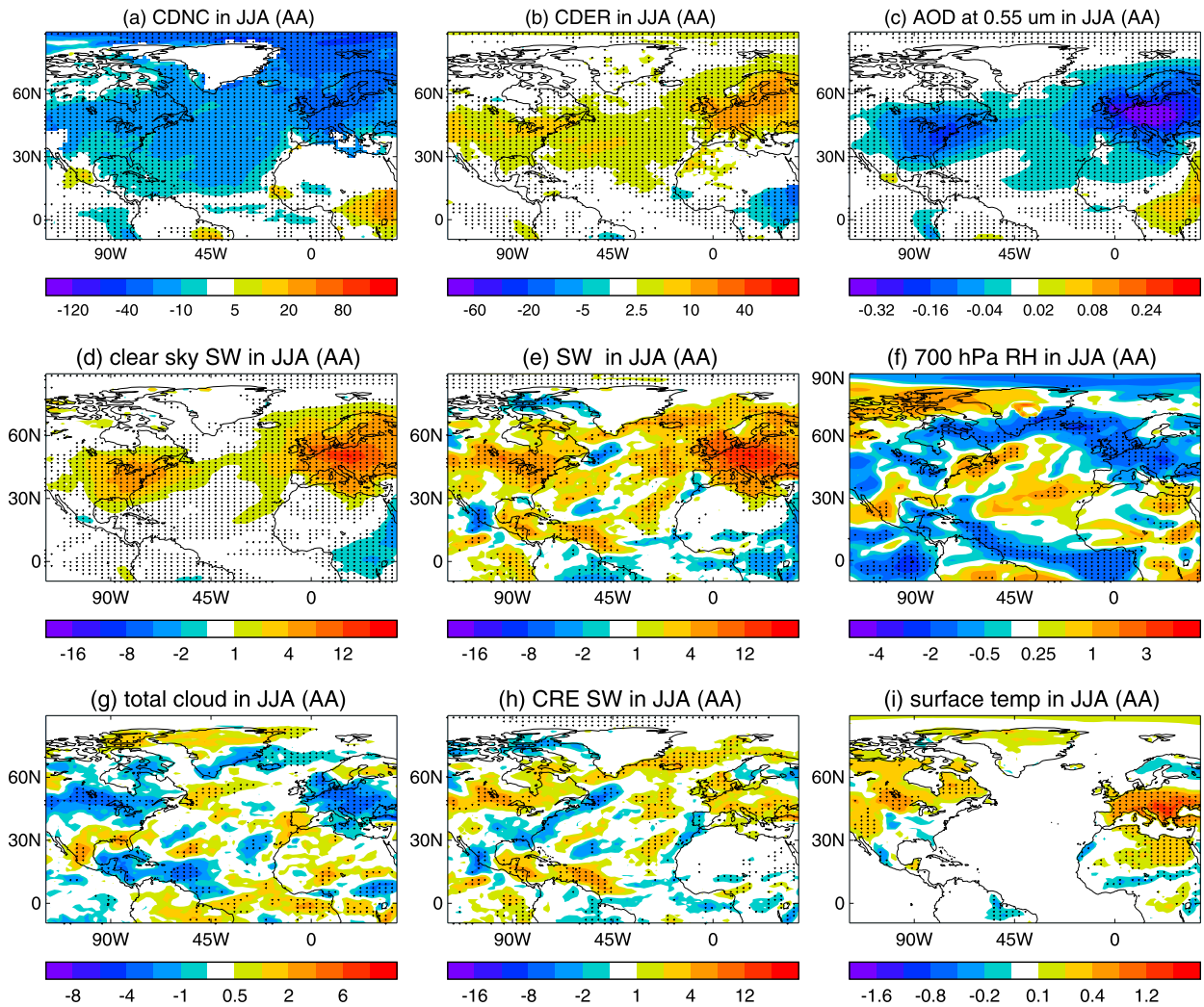
FIG. 6. Simulated climatological seasonal mean responses in JJA to AA emission changes ( SSTAA - -SST ): (a) cloud droplet number concentration (CDNC), (b) cloud droplet effective radius (CDER), (c) AOD at 0.55 \mu\text{m} , (d) surface clear-sky SW radiation, (e) surface SW radiation, (f) relative humidity at 700 hPa (%), (g) cloud fraction (%), (h) surface shortwave cloud radiative effect (CRE SW), and (i) surface temperature ( ^{\circ}\text{C} ). Radiation is positive downward. Changes in CDNC and CDER are percentage changes relative to the experiment CON. Dots highlight regions where differences are statistically significant at 10% level based on the two-tailed Student's t test.
