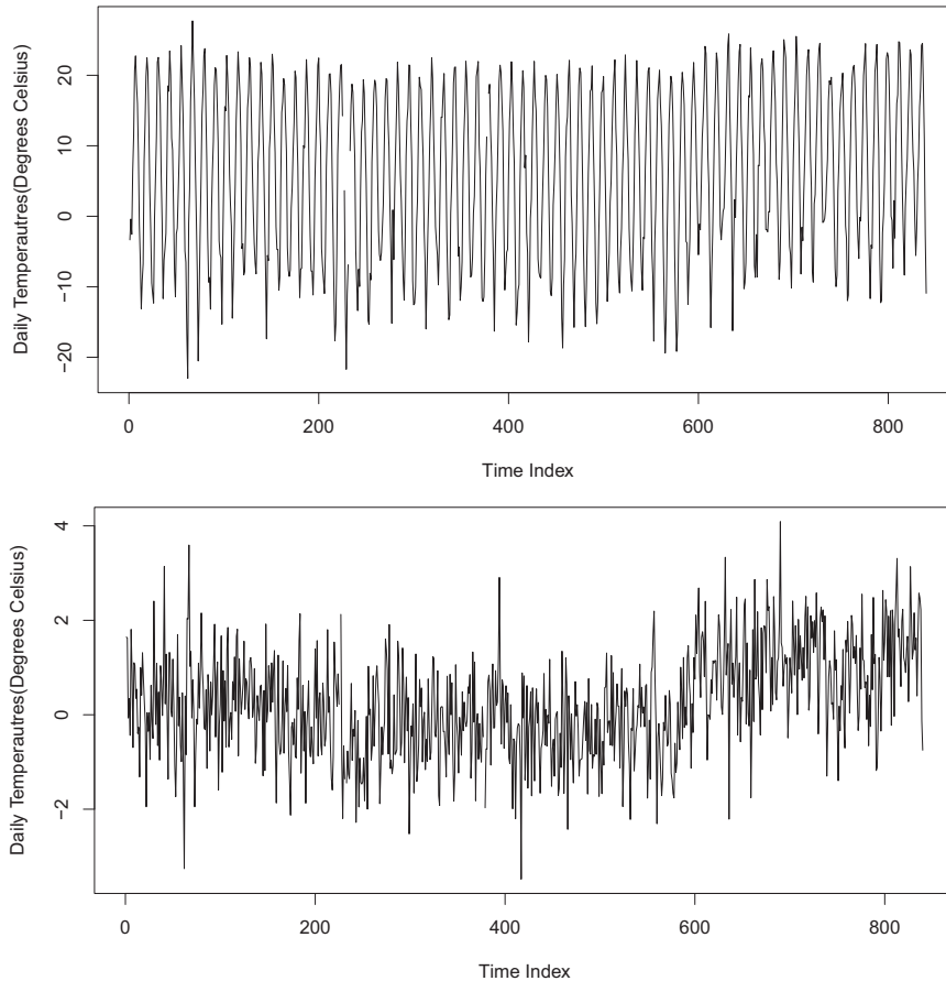
FIG. 3. The Mott series with an artificial mean change of 2^{\circ}\text{C} added after time 600, showing (a) raw data and (b) the series in (a) after the seasonal cycle has been estimated and removed.
