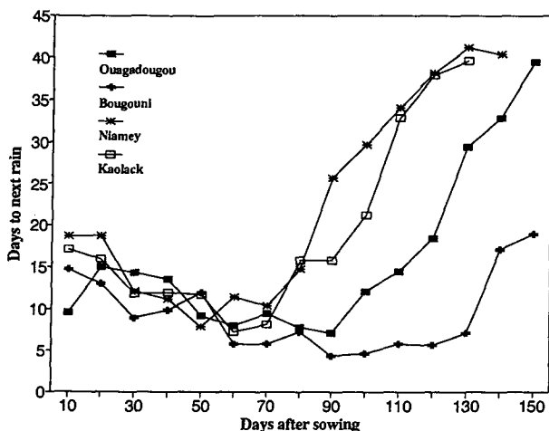
FIG. 5. Length of dry spells for 10-mm rainfall threshold at 90% probability for four locations in West Africa.
