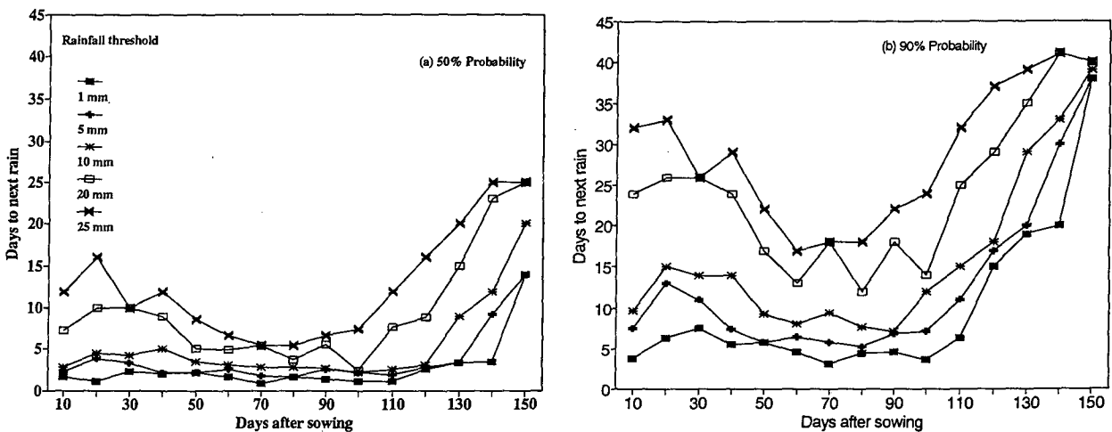
FIG. 1. Number of days until next rainfall greater than the threshold values at (a) 50% probability and (b) 90% probability at Ouagadougou, Burkina Faso.
