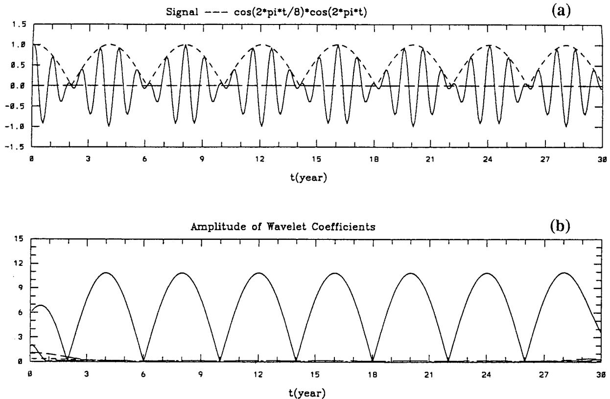
FIG. 4. Upper panel: signal of \cos(2\pi t/8)\cos(2\pi t) . Solid line: signal. Short-dashed line: envelope of the signal. Lower panel: modulus of wavelet coefficients. ---○---: a = 0.5 . Solid line: a = 1 . Long-dashed line: a = 2 . Short-dashed line: a = 4 .
