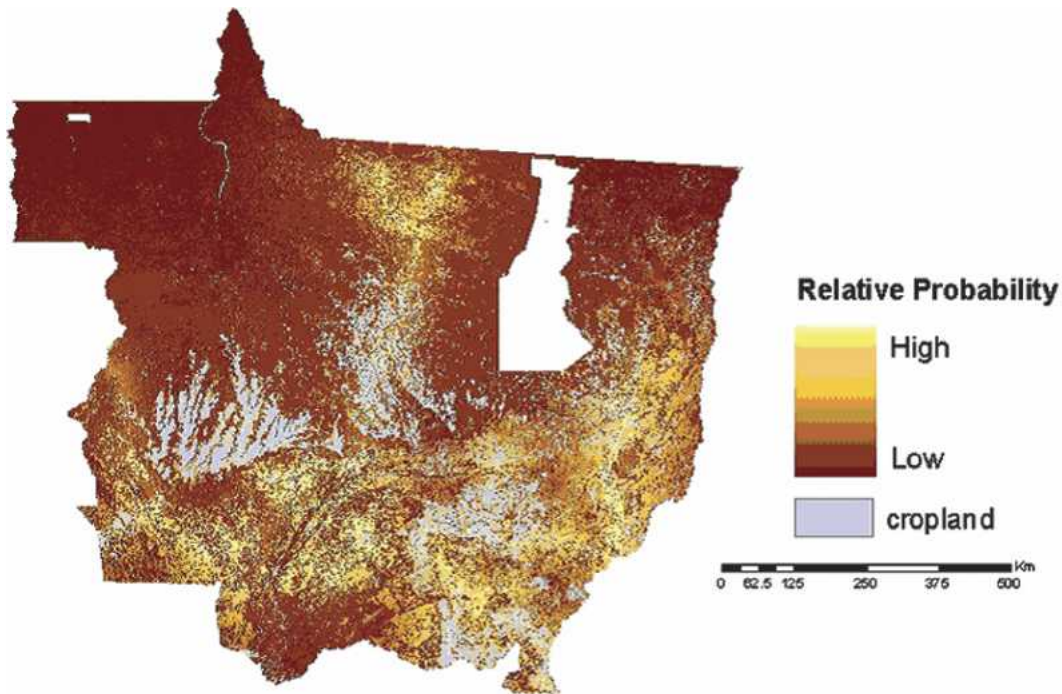
Figure 8. Probability of conversion to mechanized agriculture, based on logistic regression model of physical variables. White polygons are reserve lands excluded from the analysis, and blue pixels are those already classified as cropland as of 2003.
