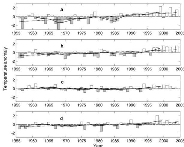
FIG. 3. Change in regional average seasonal mean temperature anomalies ( ^{\circ}\text{C} ) over the EC region from 1956 to 2004. The dashed line indicates linear trend and the curved line indicates the 11-yr Gaussian smoothed series for (a) winter, (b) spring, (c) summer, and (d) autumn.
