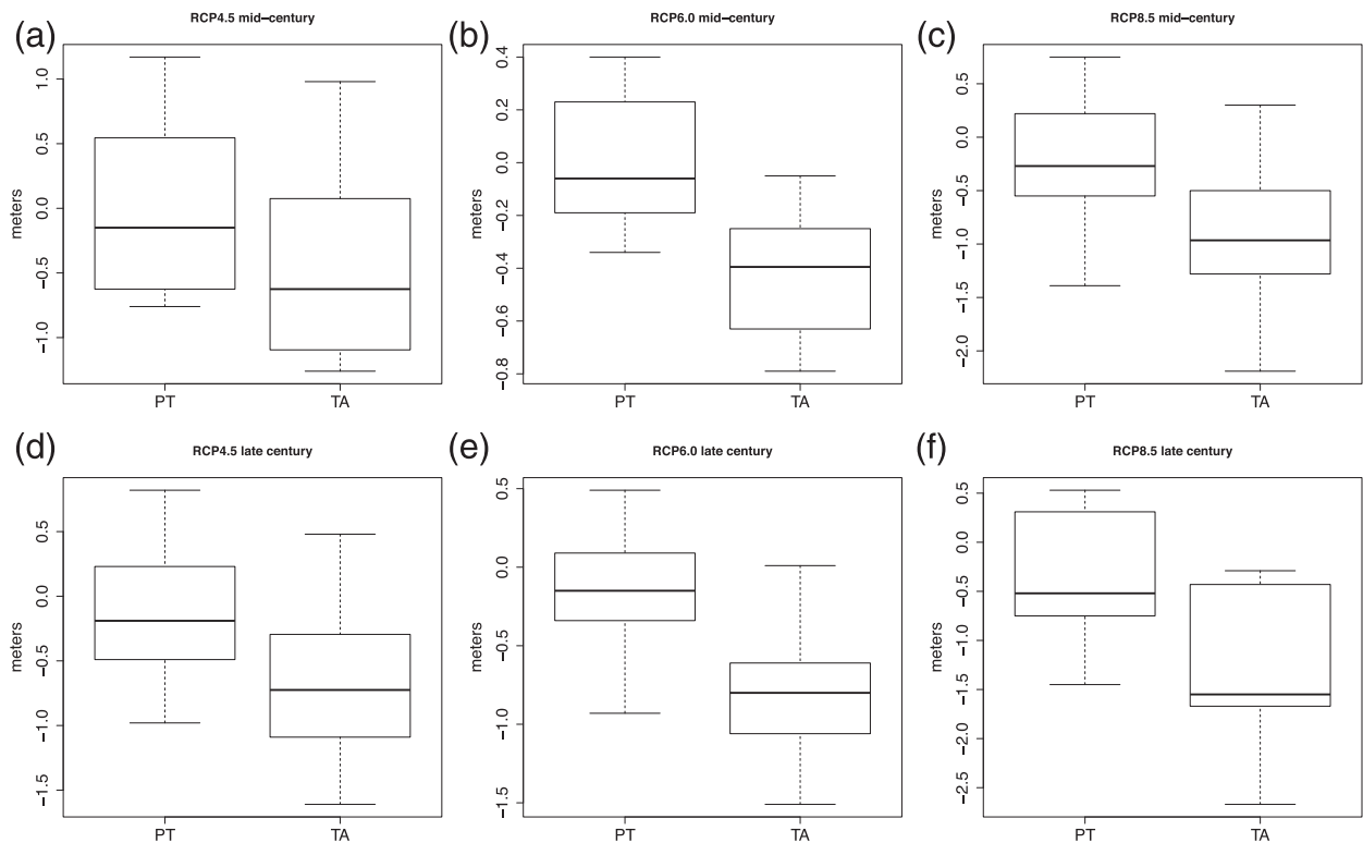
FIG. 3. Lake Michigan–Huron water levels represented using the TA and PT methods for subsets of the GCM realizations. Note that the scale differs among the panels. (a) Mid-twenty-first century for RCP 4.5, (b) mid-twenty-first century for RCP 6.0, (c) mid-twenty-first century for RCP 8.5, (d) late twenty-first century for RCP 4.5, (e) late twenty-first century for RCP 6.0, and (f) late twenty-first century for RCP 8.5. Each data point used in creating the plots represents an individual GCM realization.
