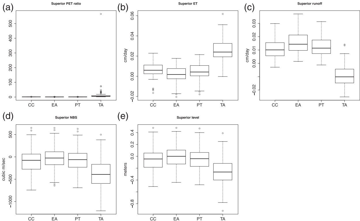
FIG. 1. Box-and-whisker plots of variables averaged over the Lake Superior basin and over the entire year, generated by GCM outputs in combination with LBRM using the TA, CC, PT, and EA methods. (a) Ratio of PET for future and historical time periods (land only), (b) ET for future minus historical time periods ( \text{cm day}^{-1} ; land only), (c) runoff for future minus historical time periods ( \text{cm day}^{-1} ), (d) net basin supply for future minus historical time periods ( \text{m}^3 \text{s}^{-1} ), and (e) lake level for future minus historical time periods (m). Each data point used in creating the plots represents an individual GCM realization.
