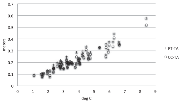
FIG. 4. Scatterplot of the difference in lake level (m) for Lake Superior, PT minus TA (plus signs) and CC minus TA (circles) vs change in air temperature. Each data point represents an individual GCM realization.
