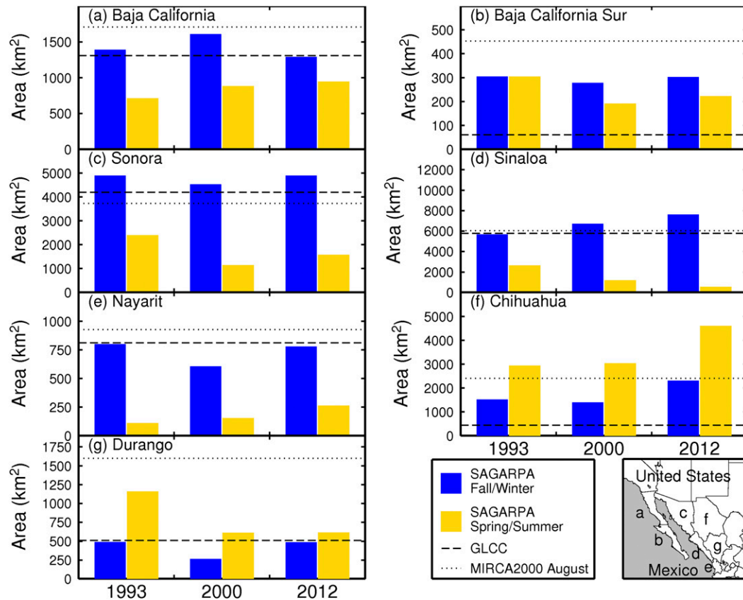
FIG. 1. Comparison of seasonal irrigated areas from government records (SAGARPA 2016), areas of irrigated cropland pixels from the GLCC classification (Loveland et al. 2000), and seasonal irrigated areas from MIRCA2000 (Portmann et al. 2010) for seven states in Mexico (locations shown in the inset map) for years 1993, 2000, and 2012. Areas of irrigated perennial crops are included in both seasons in SAGARPA bars.
