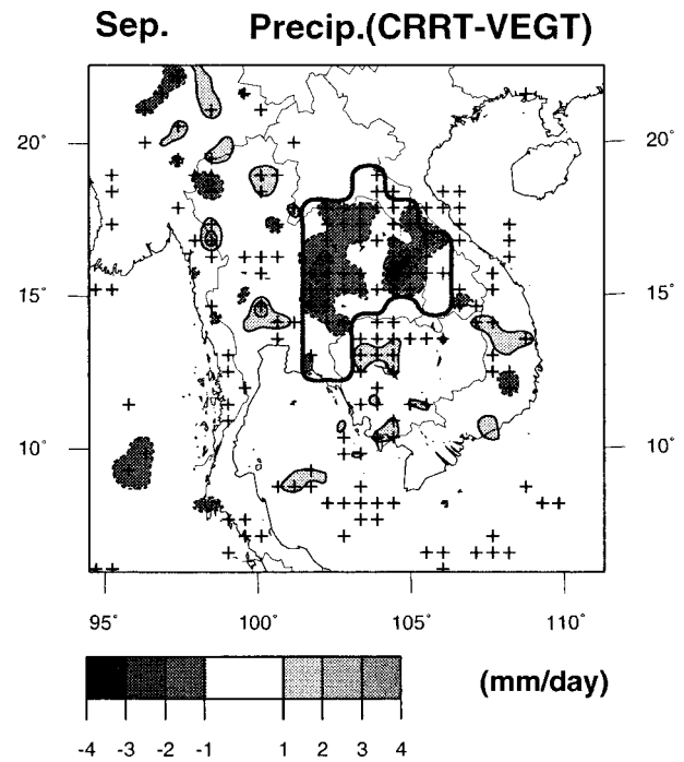
FIG. 17. As in Fig. 13, but for (CRRT - VEGT).
