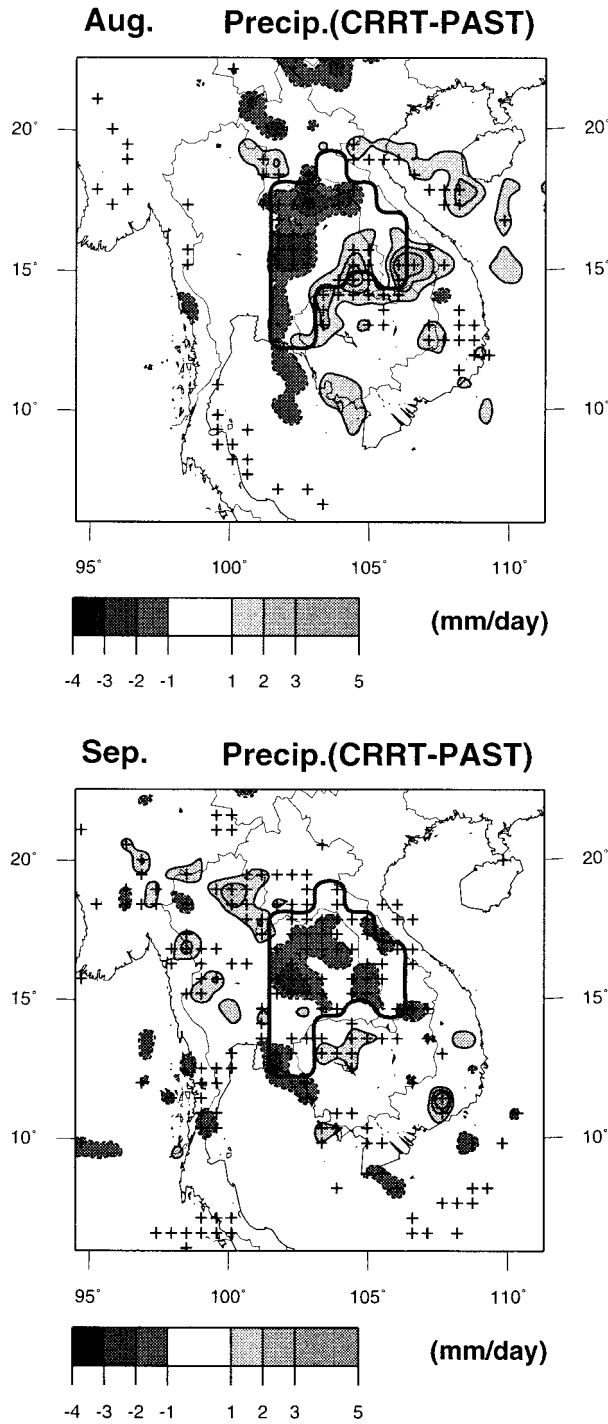
FIG. 13. Change in simulated precipitation for (CRRT - PAST) in (top) Aug and (bottom) Sep. The cross mark in this figure denotes the grid points that are statistically significant at the 95% level as determined by the Student's t test.
