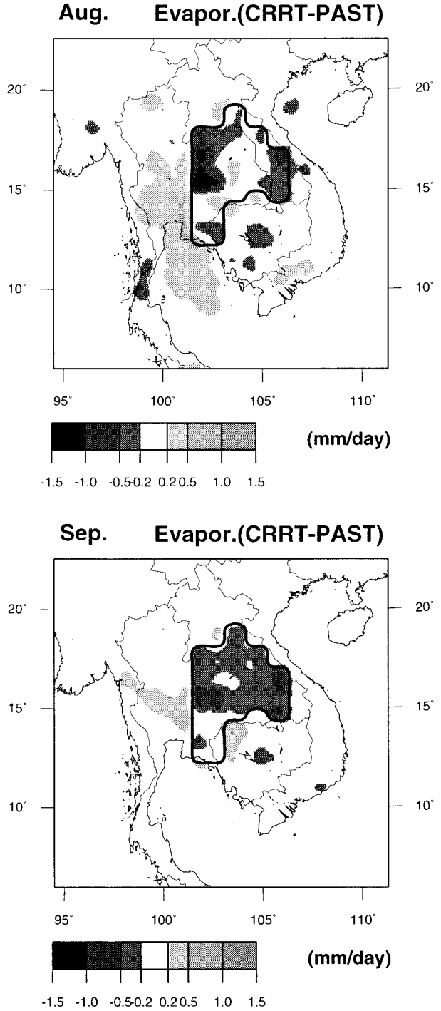
FIG. 14. Change in simulated evaporation for (CRRT - PAST) in (top) Aug and (bottom) Sep.
