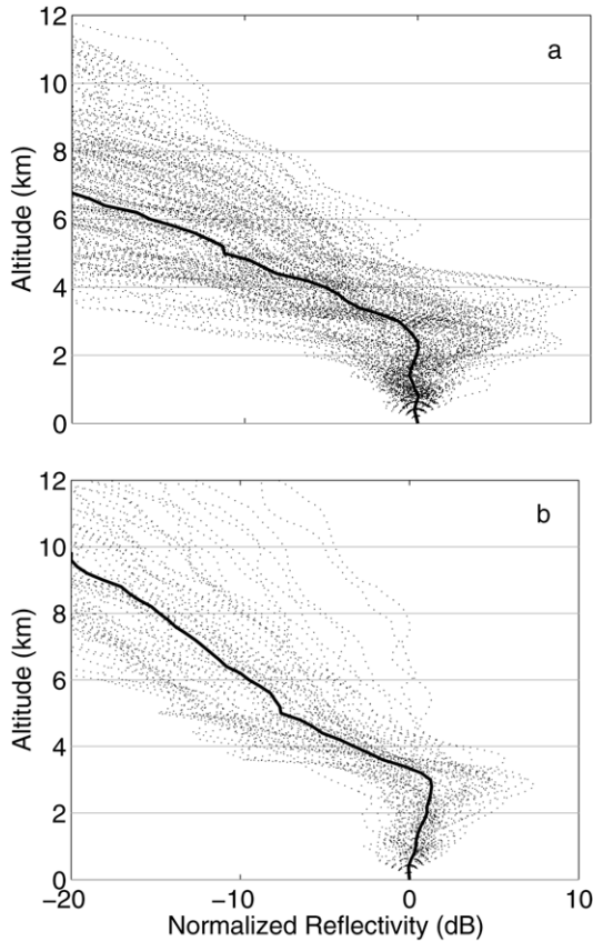
FIG. 7. Conditional sample of locally identified VPRs obtained between 60 and 90 km from the radar. (a) VPR obtained on region of analysis for which radar data at 0.5^\circ reported an average rainfall between 0.75 and 1.25 \text{ mm h}^{-1} . (b) VPR obtained on region of analysis for which radar data at 0.5^\circ reported an average rainfall between 9.50 and 10.50 \text{ mm h}^{-1} .
