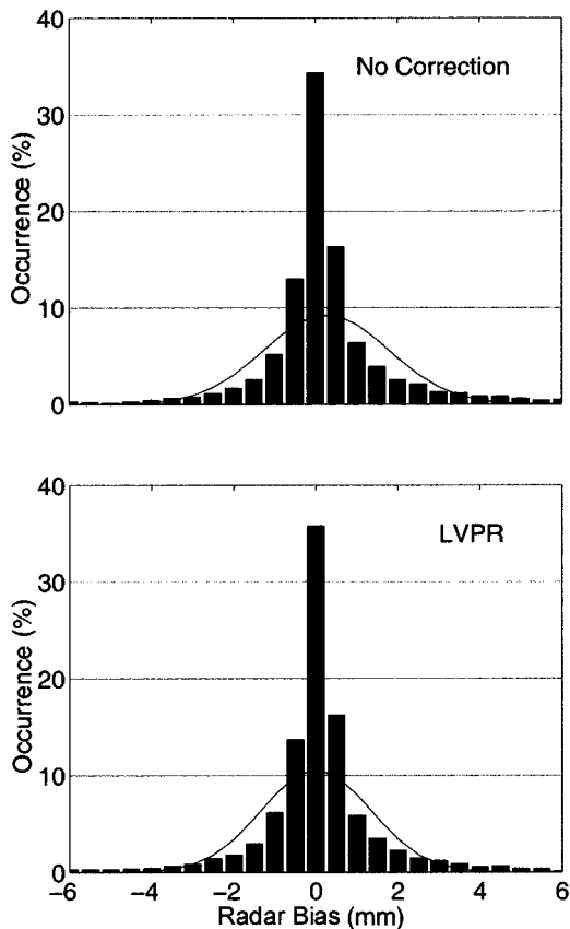
FIG. 11. Histogram of differences between radar and gauge hourly rainfall accumulation. The continuous line corresponds to the theoretical normal distribution having the same mean and variance as the studied sample.
