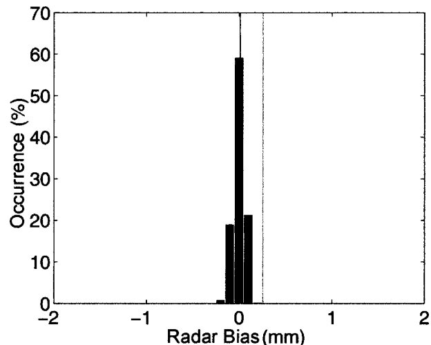
FIG. 12. The sampling distribution of the bias based on a resampling experiment using sample size of 1000. The gray vertical line shows the bias for the uncorrected data. The dark thin vertical line shows the bias obtained by the LVPR method.
