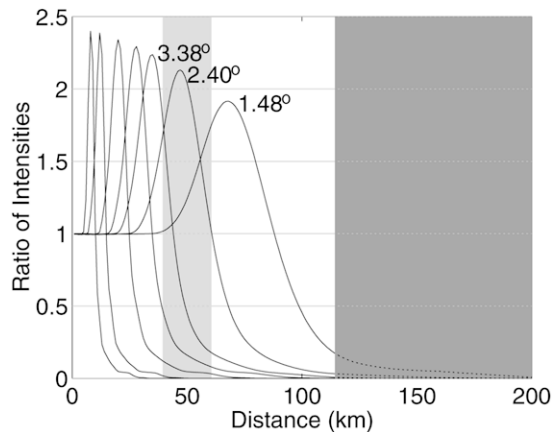
FIG. 2. Example of ratio curves of radar data simulated using the VPR shown in Fig. 1b. The light-shaded region corresponds to one 20-km interval used in LVPR-correction calculations. The dark-shaded region denotes distance over which no VPR corrections should be made, because the lowest angle ( 0.5^\circ ) is no longer a good reference.
