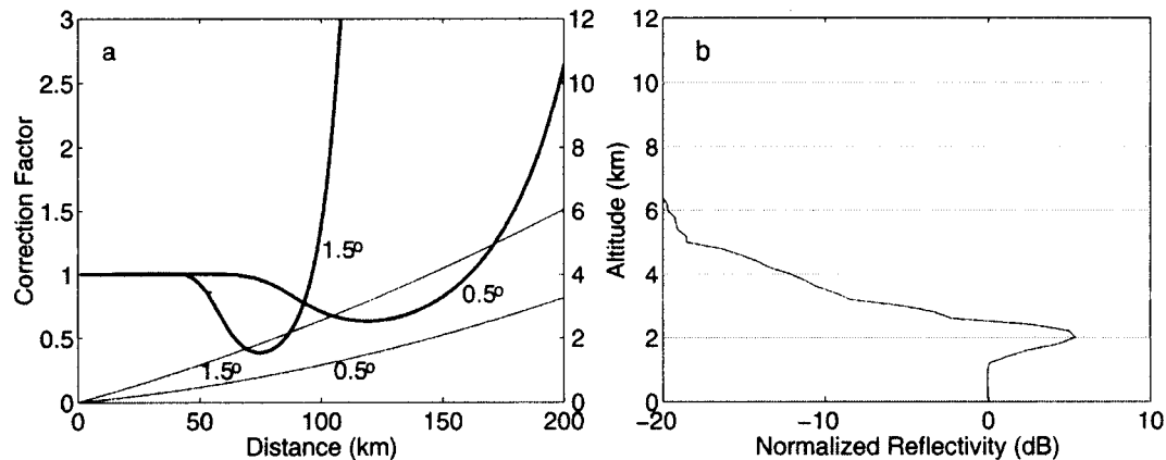
FIG. 1. (a) Illustration of VPR correction curves for two elevation angles associated with (b) an arbitrary vertical profile of reflectivity. In (a), the light lines show the altitude of the beam axis, and the dark lines are the correction factors.
