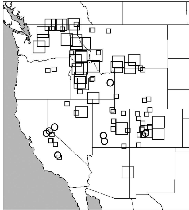
FIG. 3. Linear trends (correlations with time) in the Julian date when 50% of total annual runoff occurs, 1950–2003. Squares indicate trends to earlier dates and circles indicate trends to later dates. Large symbols indicate trends that are significant at a 90% confidence level.
