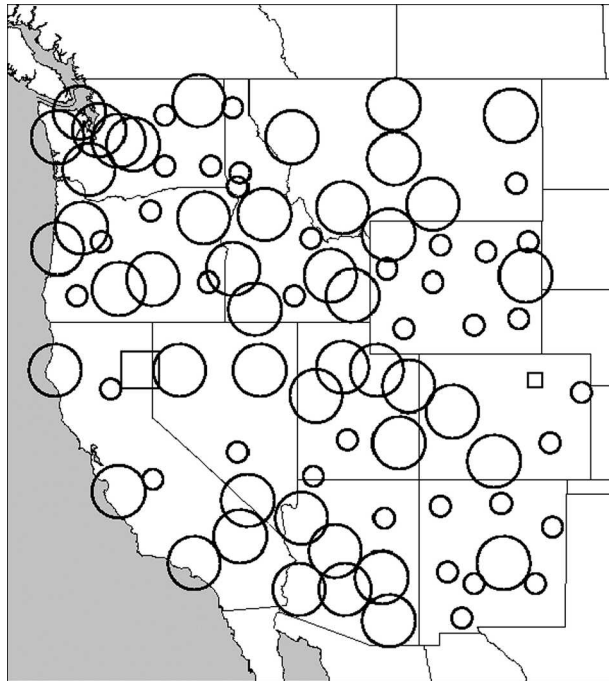
FIG. 6. Linear trends in Apr–Jul climate division temperature, 1950–2003. Squares indicate decreasing trends and circles indicate increasing trends. The large symbols indicate trends that are significant at a 95% confidence level.
