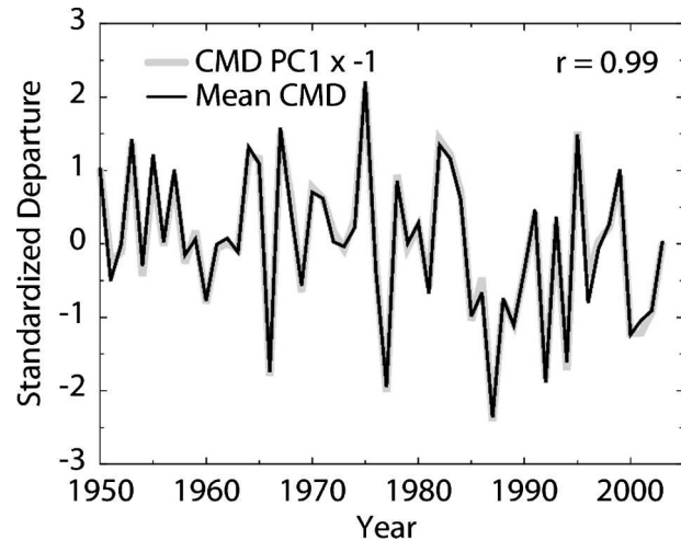
FIG. 5. Scores (gray line) for PC1 from a principal components analysis of the time series of Julian dates when 50% of annual runoff occurs (CMD) for 84 sites in the western United States, 1950–2003 (the PC1 time series was multiplied by -1 ), and standardized departures (black line) of the mean CMD time series for the 84 sites.
