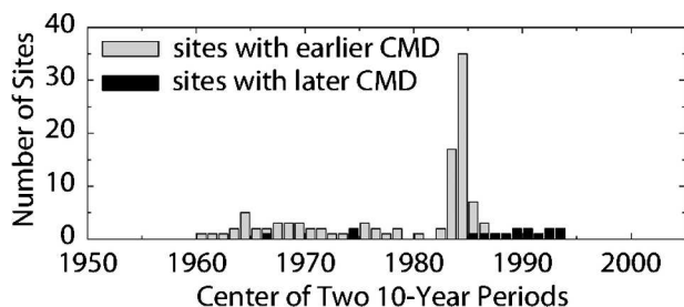
FIG. 8. Ten-year moving counts of the number of sites with statistically significant (at a 95% confidence level) increases (later timing, black bars), or decreases (earlier timing, gray bars), in the Julian date when 50% of total annual runoff occurs. The significance of the differences in mean Julian dates for sets of 10-yr moving periods was determined using a Student's t test.
