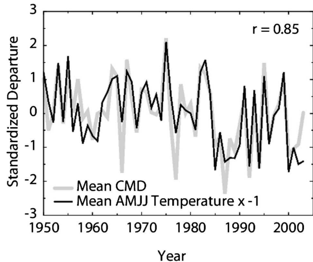
FIG. 7. Standardized departures of the mean Julian date when 50% of annual runoff occurs (CMD, averaged for 84 sites in the western United States) (gray line) and mean AMJJ temperature for the western United States (black line). The temperature time series was multiplied by -1 for easy comparison with the CMD time series.
