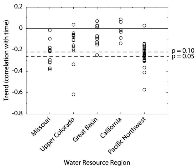
FIG. 4. Distributions of linear trends in the Julian date when 50% of total annual runoff occurs, 1950–2003, for five of the water resource regions in the western United States.
