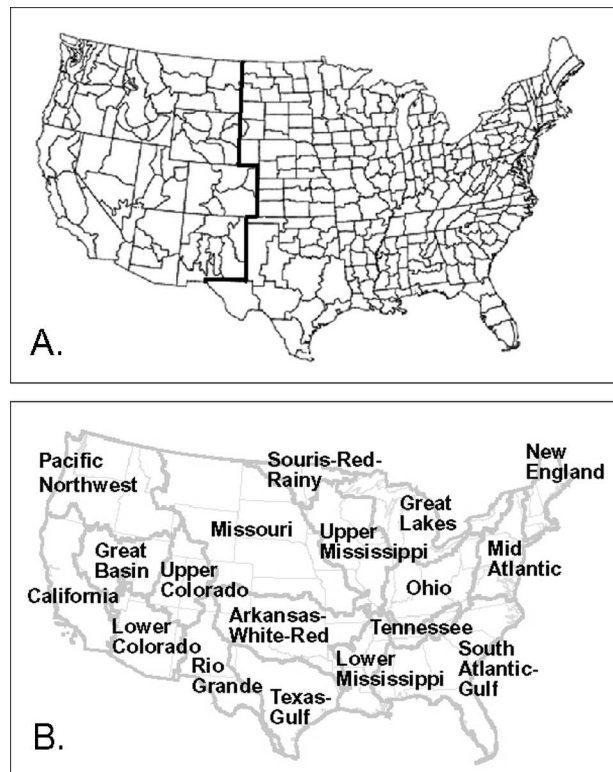
FIG. 2. (a) Climate divisions in the conterminous United States. The climate divisions to the left of the dark line were used in the analysis. (b) Water resource regions in the conterminous United States.
