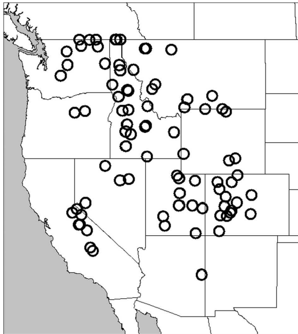
FIG. 1. Locations of streamflow sites analyzed in this study.
