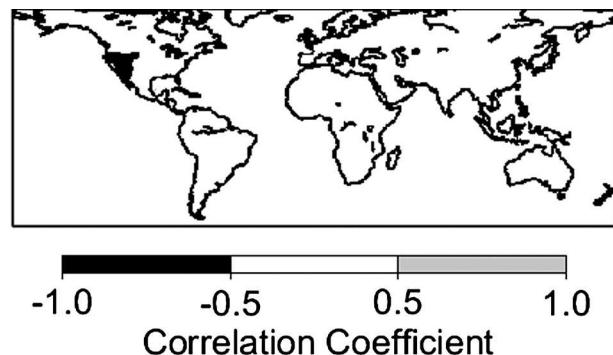
FIG. 10. Correlations between AMJJ gridded temperature and the mean Julian date (averaged for 84 sites in the western United States) when 50% of annual runoff occurs (CMD). Correlations were computed for grids with at least 30 yr of data during 1950–2003.
