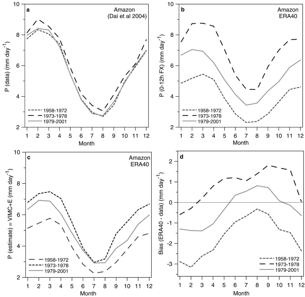
FIG. 7. Mean annual cycle of (a) observed precipitation, (b) ERA-40 0–12 h FX precipitation, (c) precipitation estimate from moisture convergence, and (d) ERA-40 precipitation bias.
