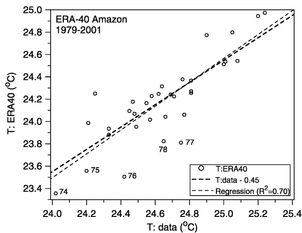
FIG. 9. ERA-40 annual mean temperature plotted against data.
