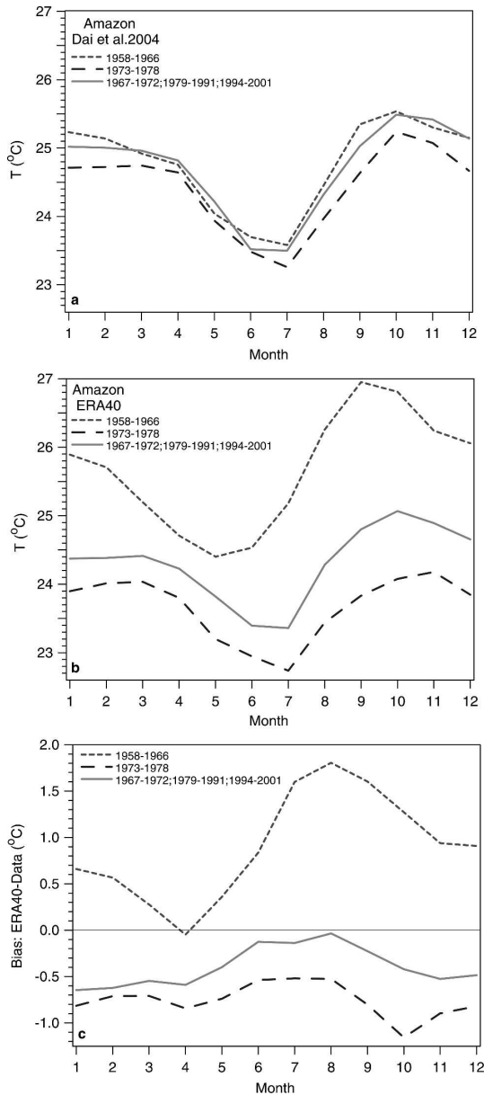
FIG. 10. Mean annual cycle of (a) observed 2-m temperature, (b) ERA-40 2-m temperature, and (c) ERA-40 2-m temperature bias.
