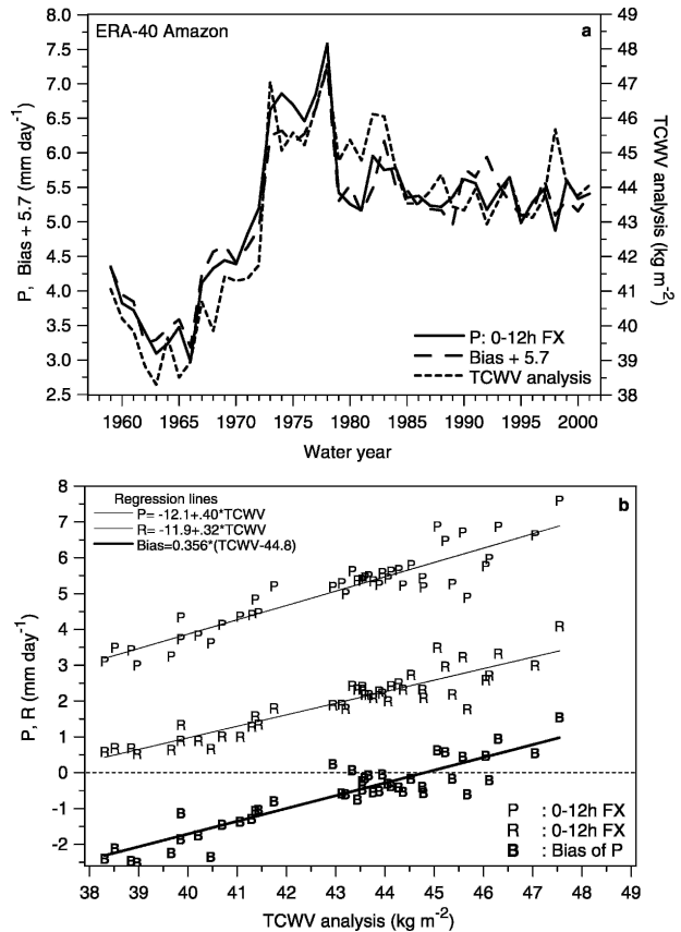
FIG. 3. (a) Annual precipitation, precipitation bias, and total column water vapor in ERA-40; (b) regression of annual precipitation, precipitation bias, and runoff against mean total column water vapor.
