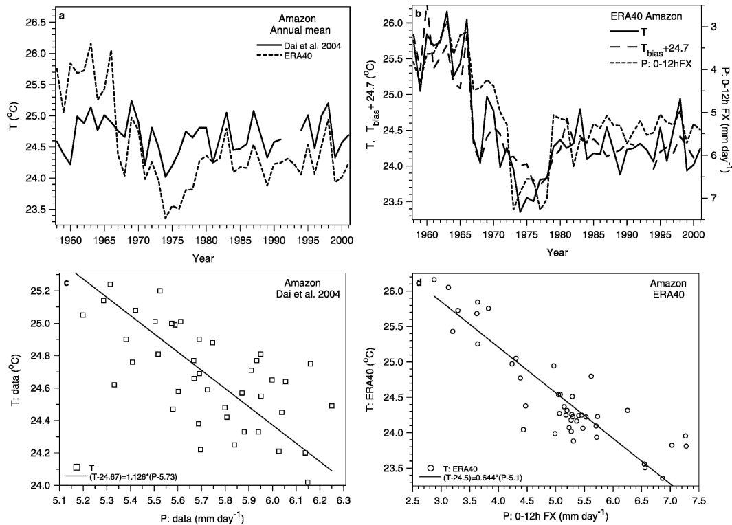
FIG. 8. (a) Comparison of annual mean observed and ERA-40 2-m temperature; (b) time series of ERA-40 2-m temperature, temperature bias, and precipitation; (c) scatterplot of observed 2-m temperature against precipitation; and (d) as (c) for ERA-40.
