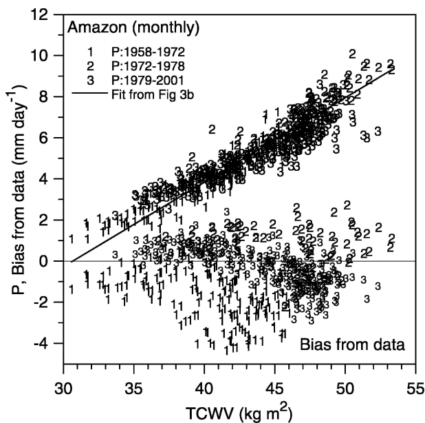
FIG. 6. Monthly precipitation and precipitation bias against TCWV for three time periods of ERA-40.
