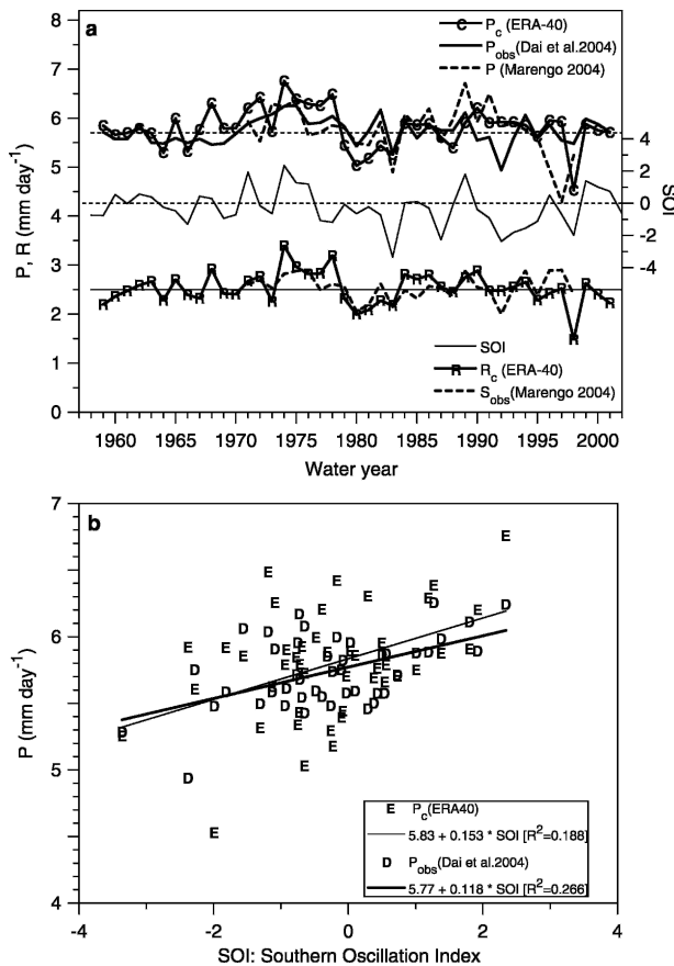
FIG. 4. (a) Comparison of corrected annual mean precipitation and runoff in ERA-40 with observations for the Amazon for water years, together with Southern Oscillation index (SOI). (b) ERA-40 P_c and Dai et al. (2004) P_{\text{obs}} against SOI (with regression lines).
