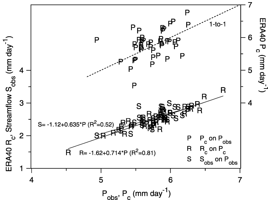
FIG. 5. ERA-40 P_c against P_{obs} (with 1-to-1 line), ERA-40 R_c against P_c , and Amazon S_{obs} against P_{obs} (with regression lines).
