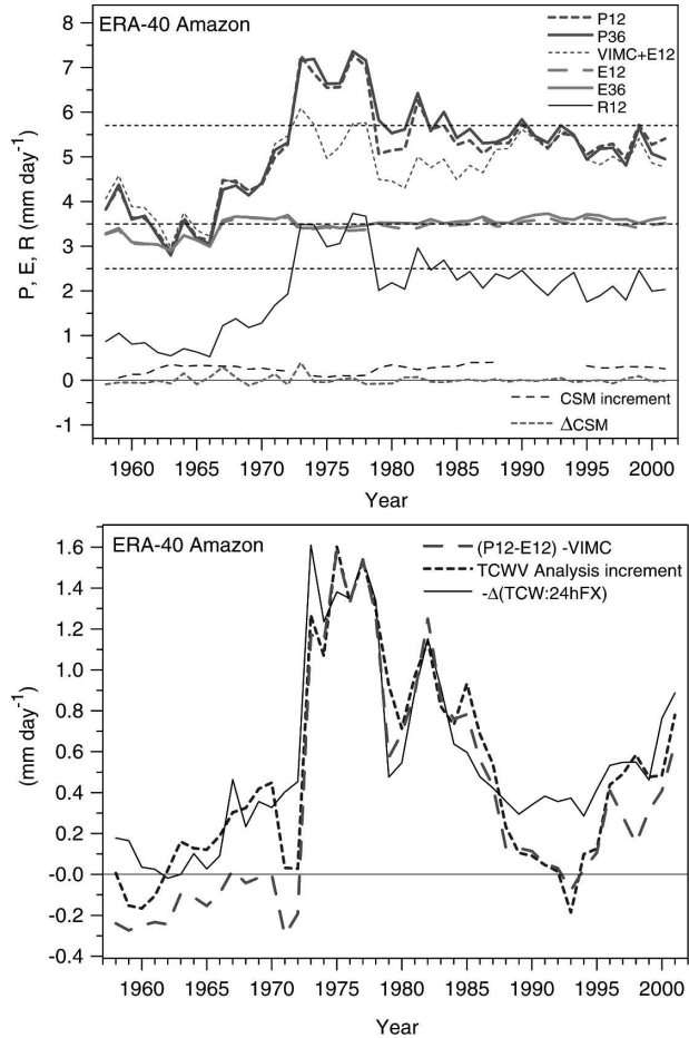
FIG. 2. (a) Terms in the surface water budget in ERA-40 for the Amazon. (b) Comparison of (P-E-VIMC) with TCW analysis increment and 24-h forecast tendency.
