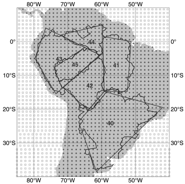
FIG. 1. ERA-40 South American basins.
