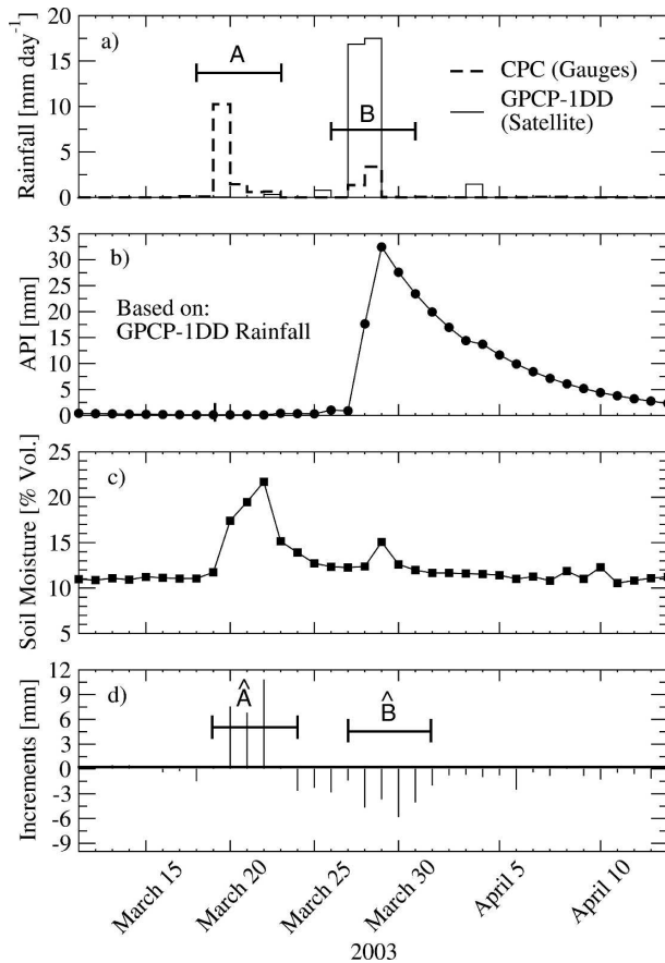
FIG. 2. Times series of daily rainfall, (b) GPCP-1DD API, (c) remotely sensed soil moisture ( TMI_{LSMEM} ), and (d) Kalman filter increments during 2003 for box 1 in Fig. 1.
