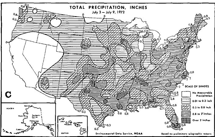
FIGURE 7.—(A) mean 700-mb contours (dam) for July 4-8, 1972; (B) departure from normal of average surface temperature ( ^{\circ}\text{F} ) and (C) total precipitation (in.) for week of July 3-9, 1972 (from Environmental Data Service and Statistical Reporting Service 1972).
