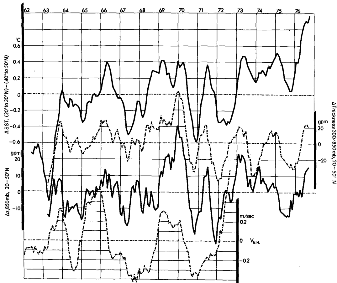
FIG. 5. Seven-month time-smoothed anomalies of Pacific SST gradients between the latitude bands 20-30°N and 40-50°N (top curve; °C scale on left side; positive values mean larger-than-normal temperature differences). Vertical lines indicate January of each respective year. The remaining curves are: atmospheric meridional thickness gradient 300-850 mb between 20 and 50°N (dashed-dotted curve, geopotential meters, scale on right side); height gradient between 20 and 50°N of the 850 mb surface (geopotential meters, scale on left side); v component of trade winds over the North Pacific (dashed-dotted curve, meters per second, scale on right side).
