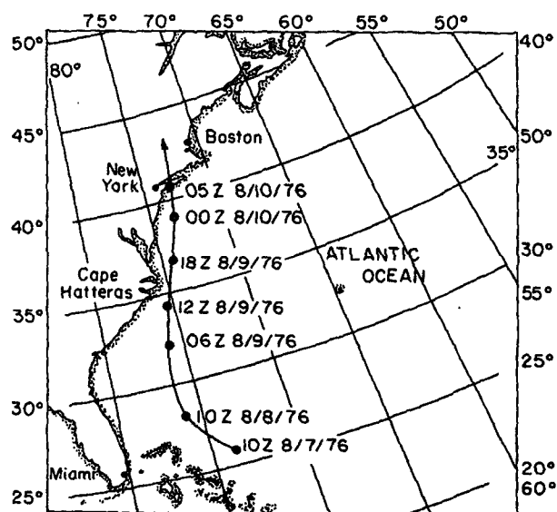
FIG. 1. Hurricane Belle storm track.
