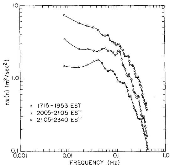
FIG. 9. Variance spectrum of horizontal velocity fluctuations during the approach and landfall of hurricane.
