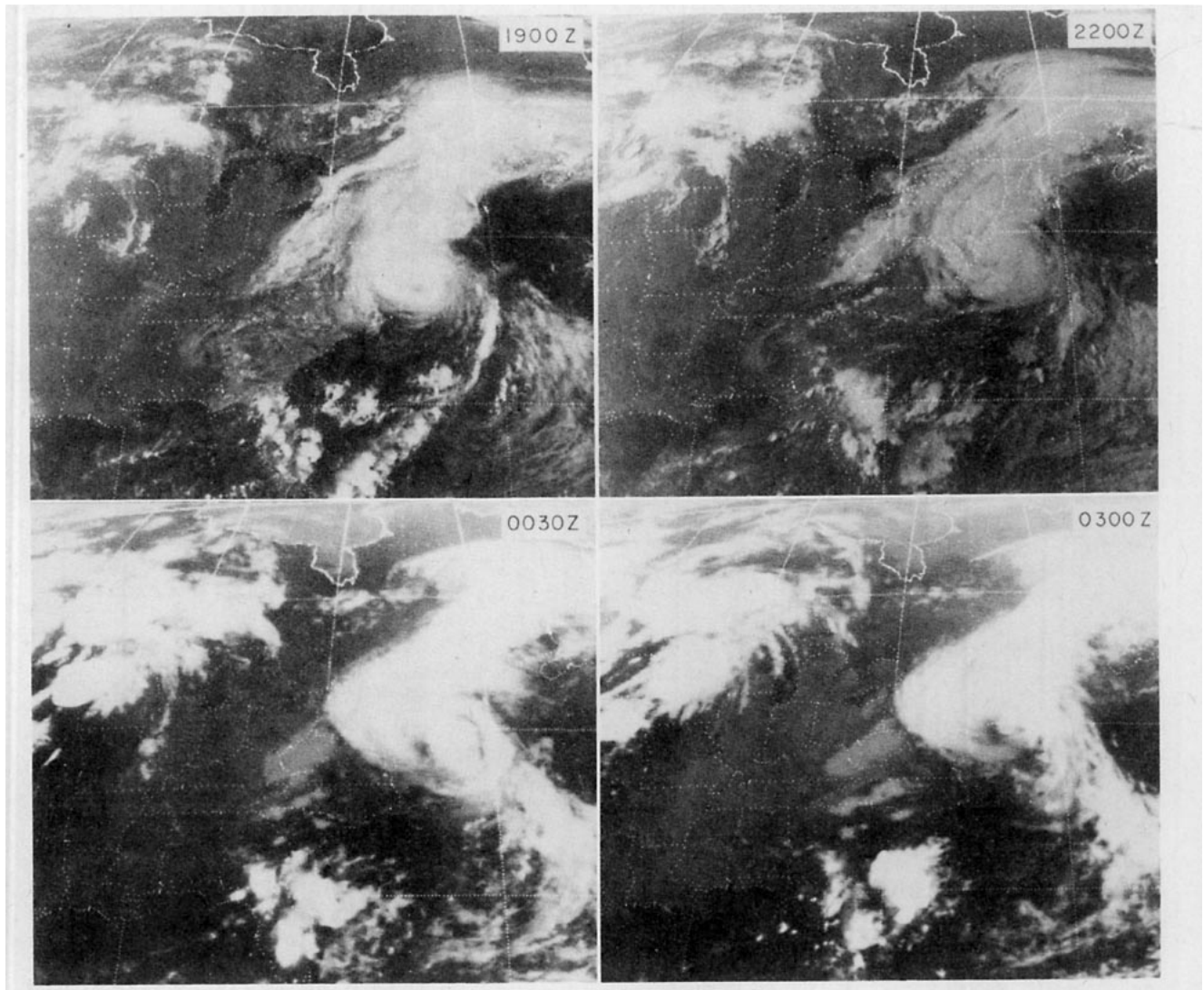
FIG. 2. Satellite pictures of Hurricane Belle. The times noted are GMT. The top two are visible (9 August) and the bottom two are infrared (10 August) views of the hurricane.
