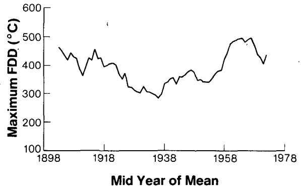
FIG. 3. Eleven-year running mean of averaged freezing degree-days (1898-1977) for the southern half Lake Michigan.
