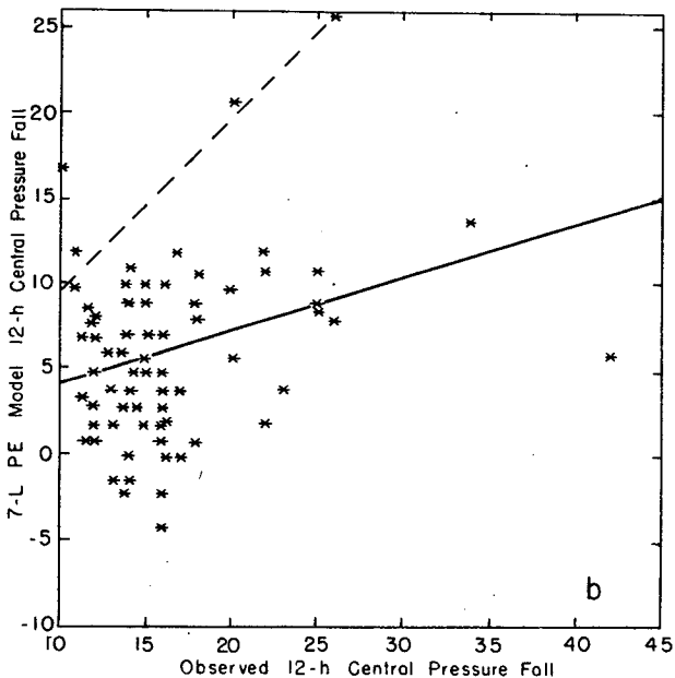
FIG. 15. Plots of observed atmospheric bombs indicating their observed 12 h central pressure fall, and the corresponding PE predicted fall at a forecast range of 12-24 h. Straight line is the least-square regression of the points. Dashed line is the perfect forecast line.
