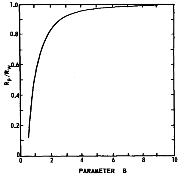
FIG. 3. The variation with B of the ratio of radius of maximum pressure gradient R_p and radius of maximum winds R_w .
