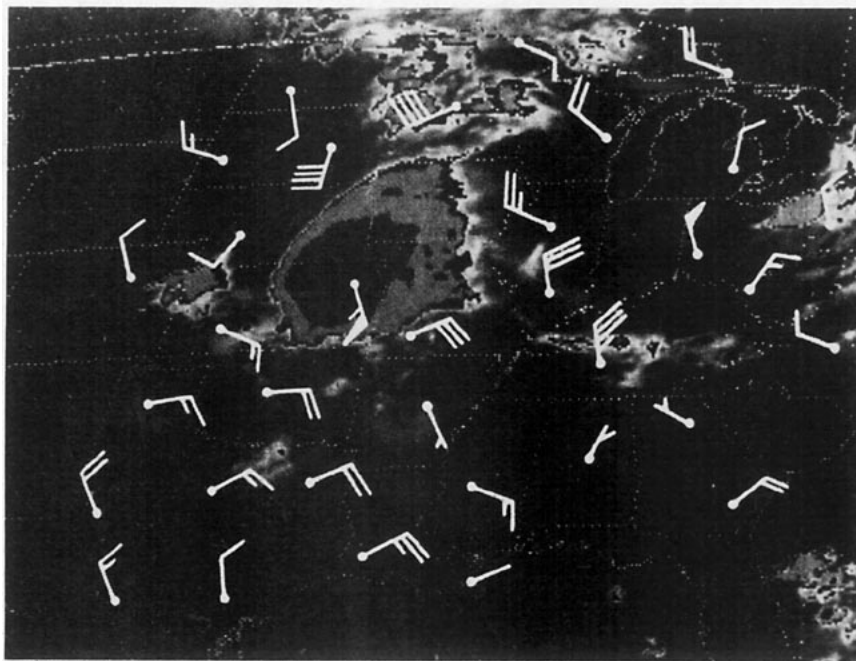
FIG. 1. Infrared satellite imagery of mesoscale convective complex at 1200 GMT 28 June 1979. Wind barbs are vector errors of the 12 h LFM predicted 200 mb wind field. Full wind barb = 5 \text{ m s}^{-1} ; flag = 25 \text{ m s}^{-1} .
