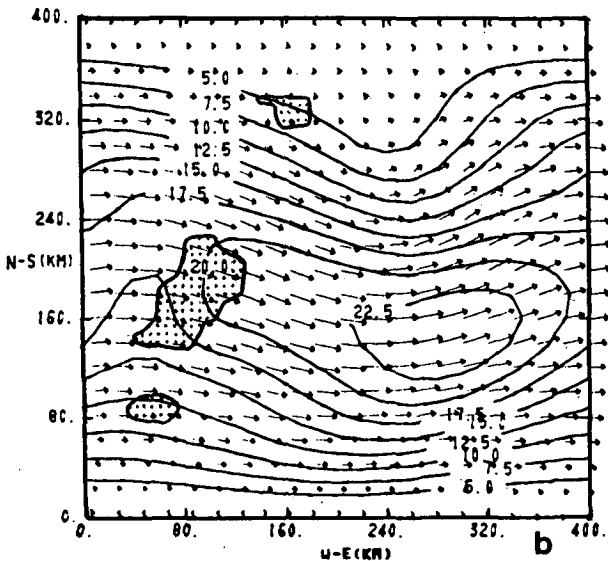
FIG. 8. Isotachs ( m s^{-1} , solid lines), wind direction (arrows) and location of active convection (stippled) at 11.8 km level 30 min after convection began. In (a) cooling by overshooting cloud tops is included; in (b) it is omitted.
