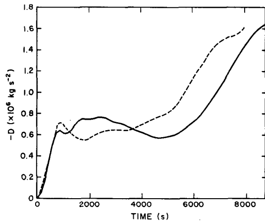
FIG. 12. Magnitude of the surface wave drag as a function of time, from this model (solid line) and from the simulation of Peltier and Clark (1979) (dashed line).
