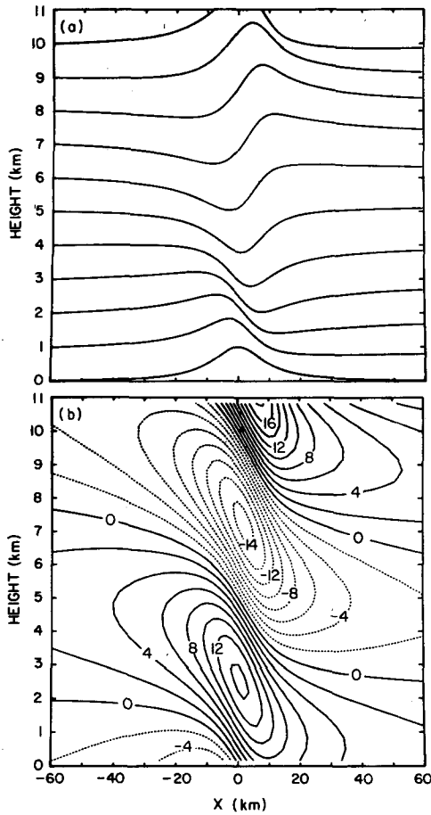
FIG. 13. (a) Streamlines and (b) horizontal velocities produced by a 1 m high mountain when RH = 0% upstream. The perturbations have been multiplied by 1000 for display; as such they constitute a linear numerical solution for a 1 km high mountain.
