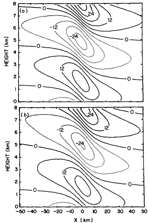
FIG. 1. (a) Steady state perturbation horizontal velocity ( m s^{-1} ) from the linear hydrostatic solution for a 1000 m high mountain. (b) Perturbation horizontal velocity ( m s^{-1} ) obtained by numerical simulation for a 1 m high mountain at \bar{u}/a = 60 ; the perturbations have been amplified by 1000.
