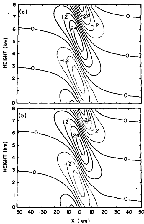
FIG. 2. As in Fig. 1, except that the fields plotted are vertical velocity ( m\ s^{-1} ).
