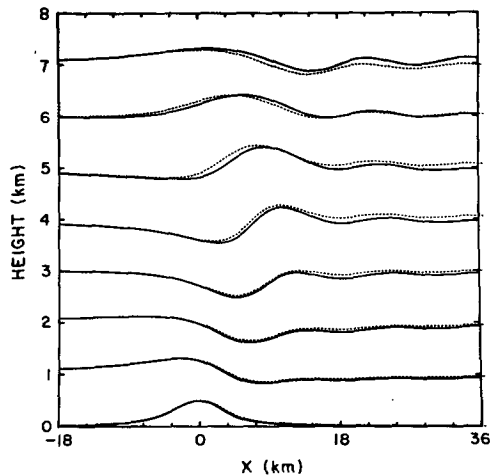
FIG. 4. Streamlines obtained from Long's solution (dashed lines), and by numerical simulation at \bar{u}t/a = 40 (solid lines).
