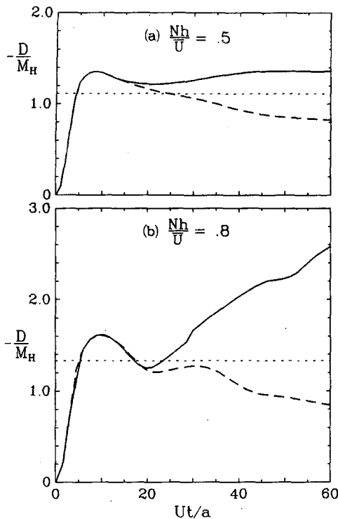
FIG. 6. Surface pressure drag, normalized by its linear hydrostatic value, as a function of time obtained from numerical simulations in which the bottom of a 1.5\lambda_z thick wave-absorbing layer is located at 1.25\lambda_z (solid line) or 1.5\lambda_z (dashed line), and Nh/\bar{u} is (a) 0.5, or (b) 0.8.
