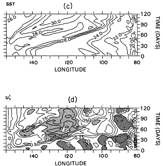
FIG. 8. Equatorial time-longitude sections of the model anomalous surface current u' , and of SST for two anomalous westerly wind patch experiments using \tau'_x = 0.05 \text{ N m}^{-2} (a and b), and \tau'_x = 0.1 \text{ N m}^{-2} (c and d). Regions where u' exceeded 0.5 \text{ m s}^{-1} are stippled on the left, and regions where u' exceeded 1.0 \text{ m s}^{-1} are stippled on the right. Negative u' regions are cross-hatched. See text for discussion.
