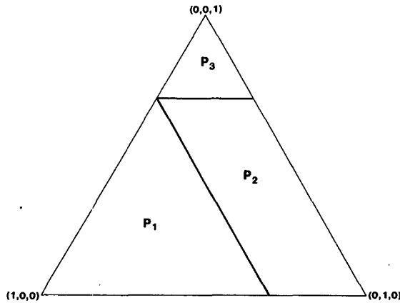
FIG. 1. The sets of climatological probabilities (p_1, p_2, p_3) for which action P_i ( i = 1, 2, 3 ) is preferred in a three-action, three-event situation in which C/L = 0.3 . Each point in (or on) the equilateral triangle corresponds to a set of possible climatological probabilities (see text for additional details).
