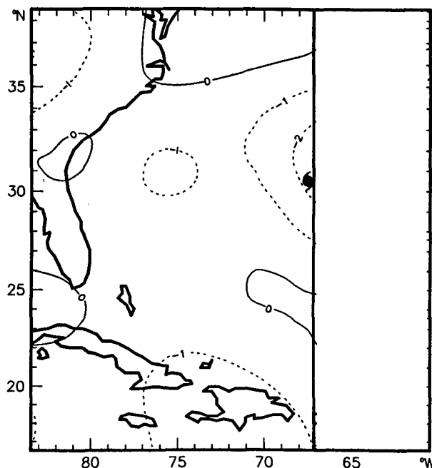
FIG. 10. As in Fig. 9 but for 500 mb temperature ( ^{\circ}\text{C} ).
